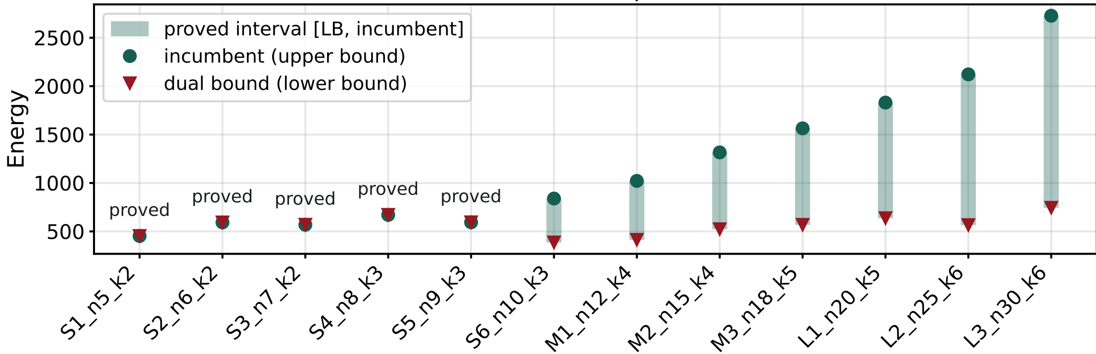
Branch & Bound: where the optimum is known to lie
