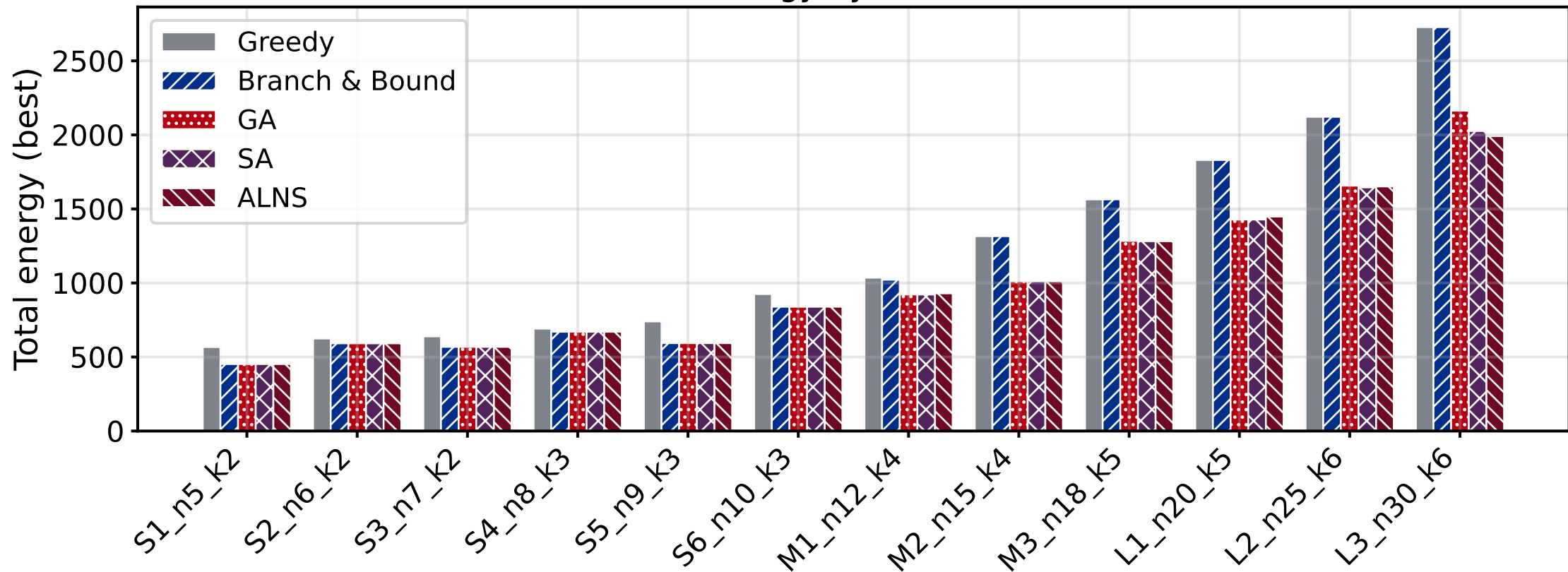
Best solution energy by method and instance
