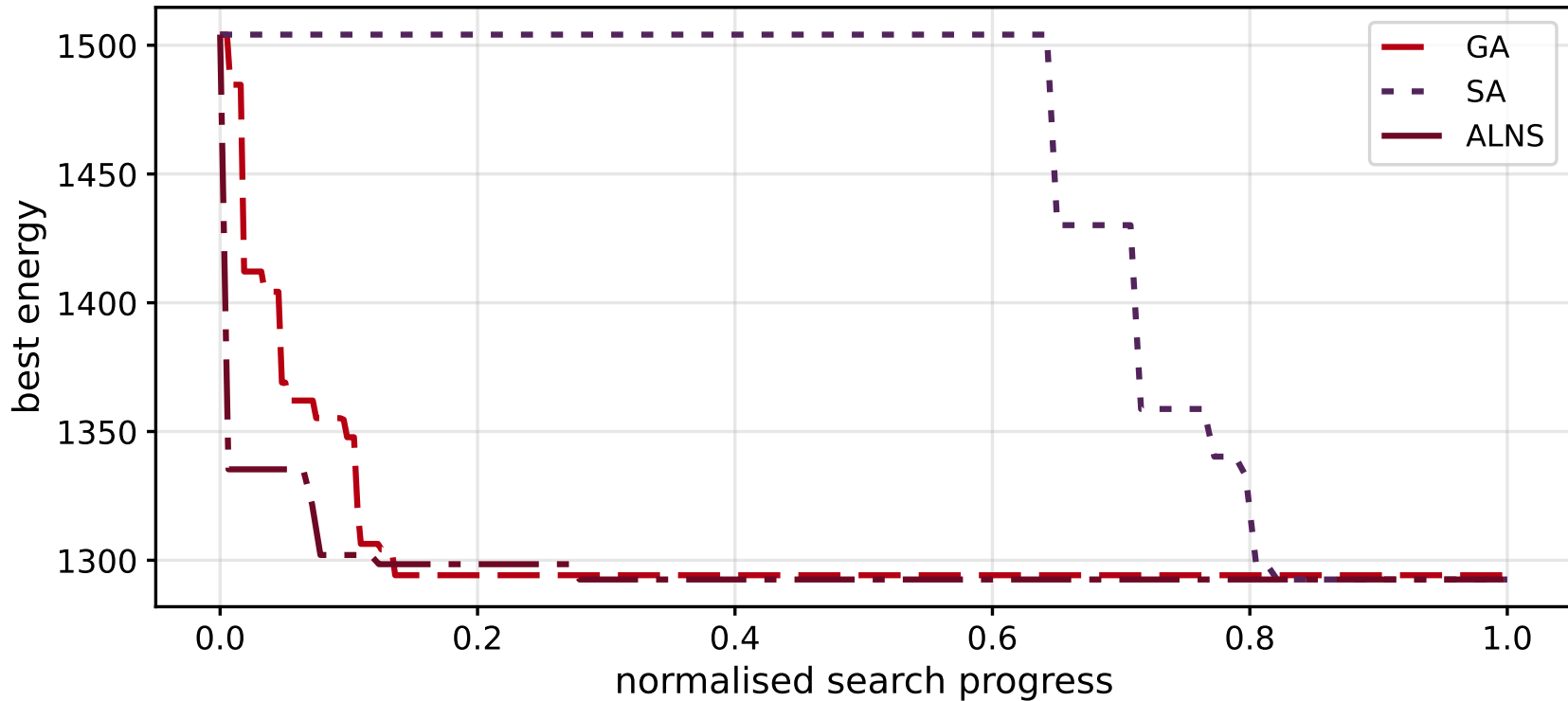
Convergence on M3_n18_k5 ( n = 18, K = 5 )
