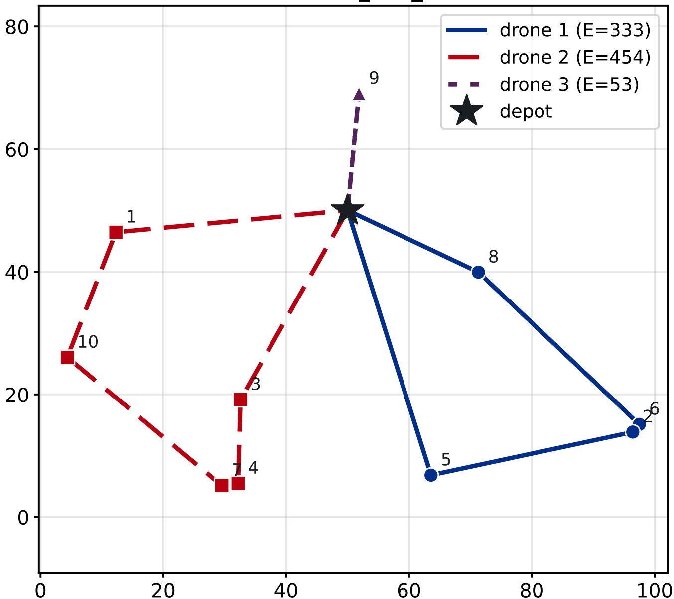
ALNS solution -- S6_n10_k3 ( E = 839 )
