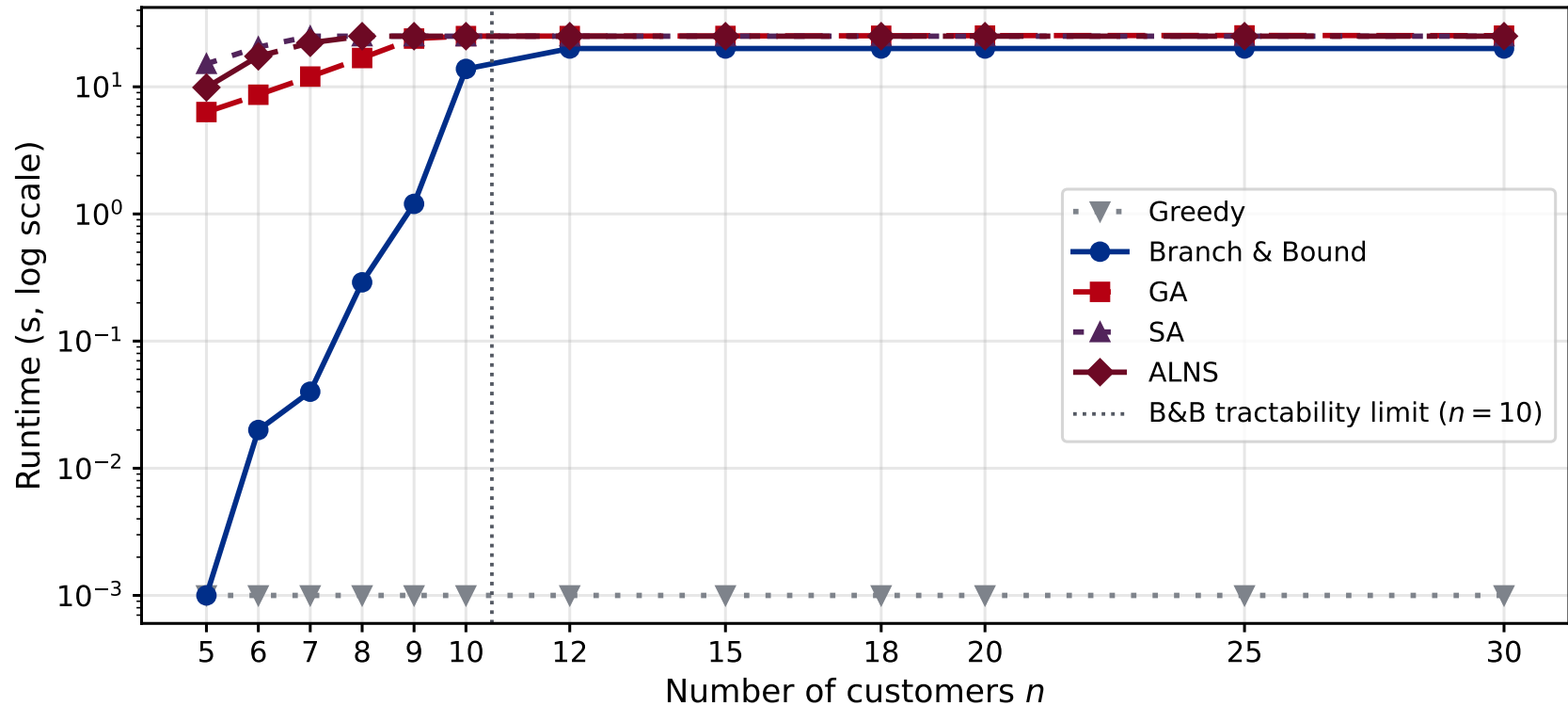
Runtime vs instance size
