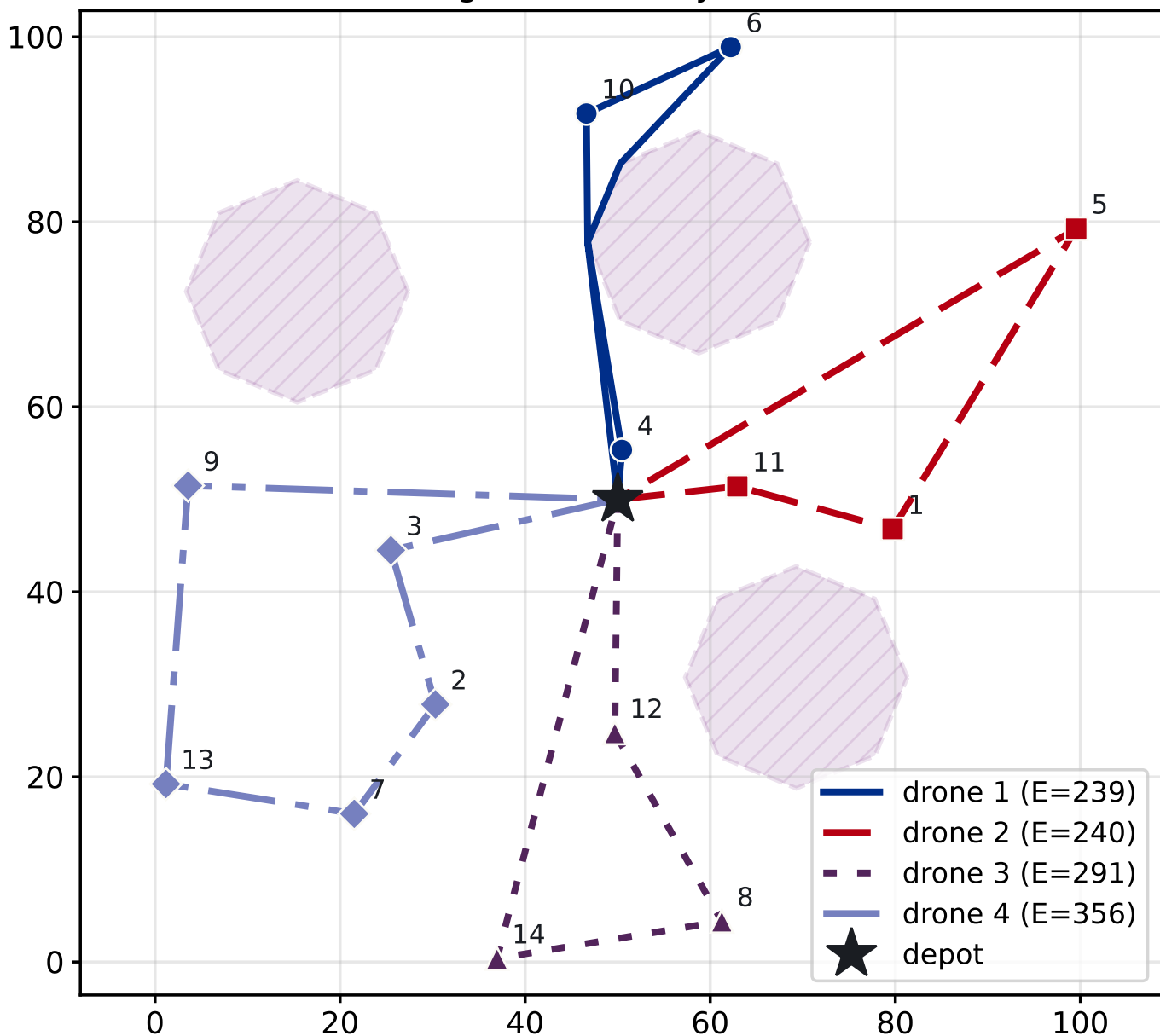
Detour routing around no-fly zones ( E = 1126 )
