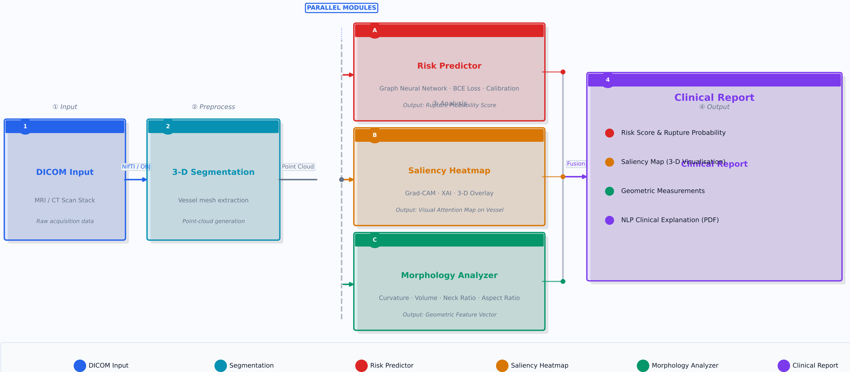
Figure 1 — Three-module architecture of the AneuXplain system (DICOM input → segmentation → three parallel modules: risk predictor, heatmap, morphology → clinical report).
