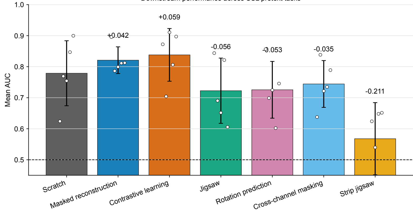
Downstream performance across SSL pretext tasks
