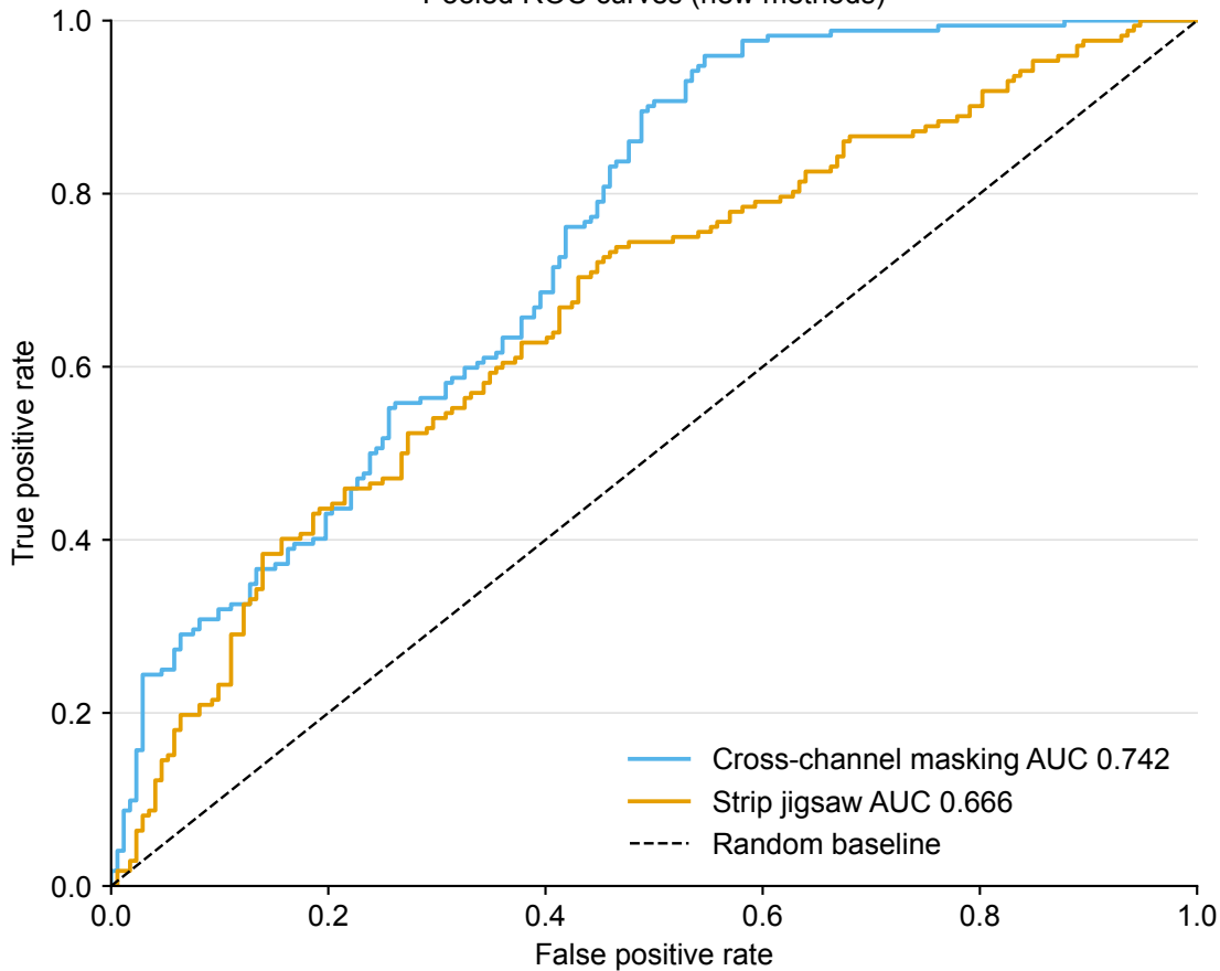
Pooled ROC curves (new methods)
