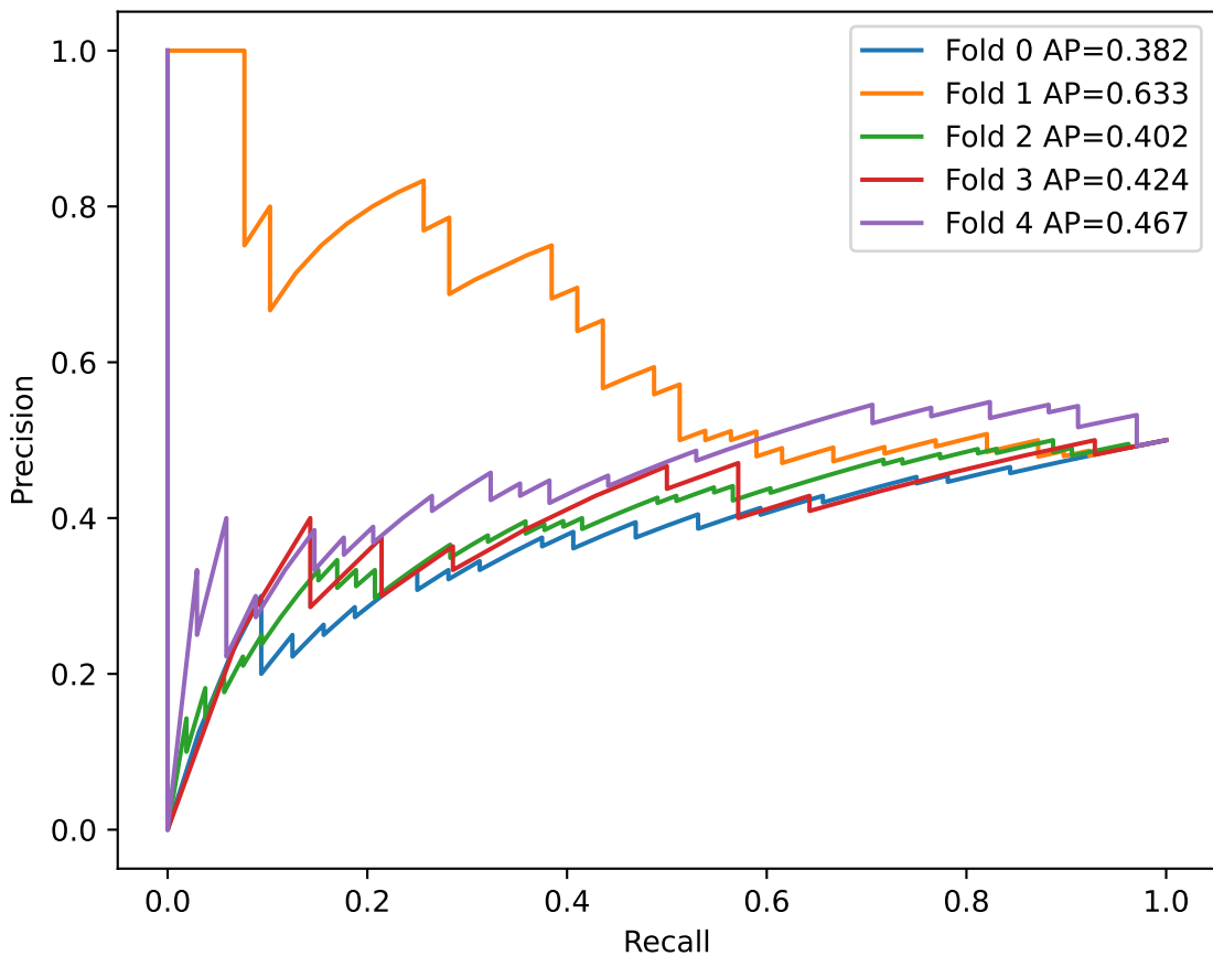
PR curves, mean AP=0.462
