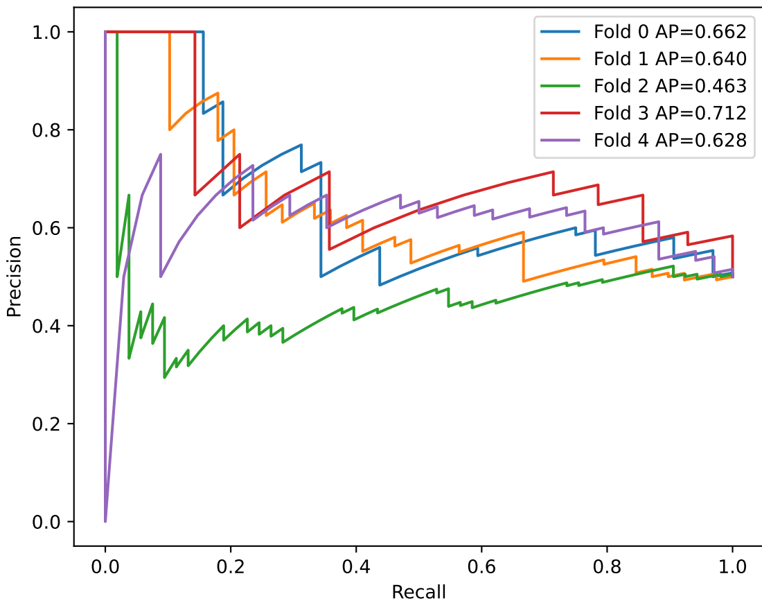
PR curves, mean AP=0.621
