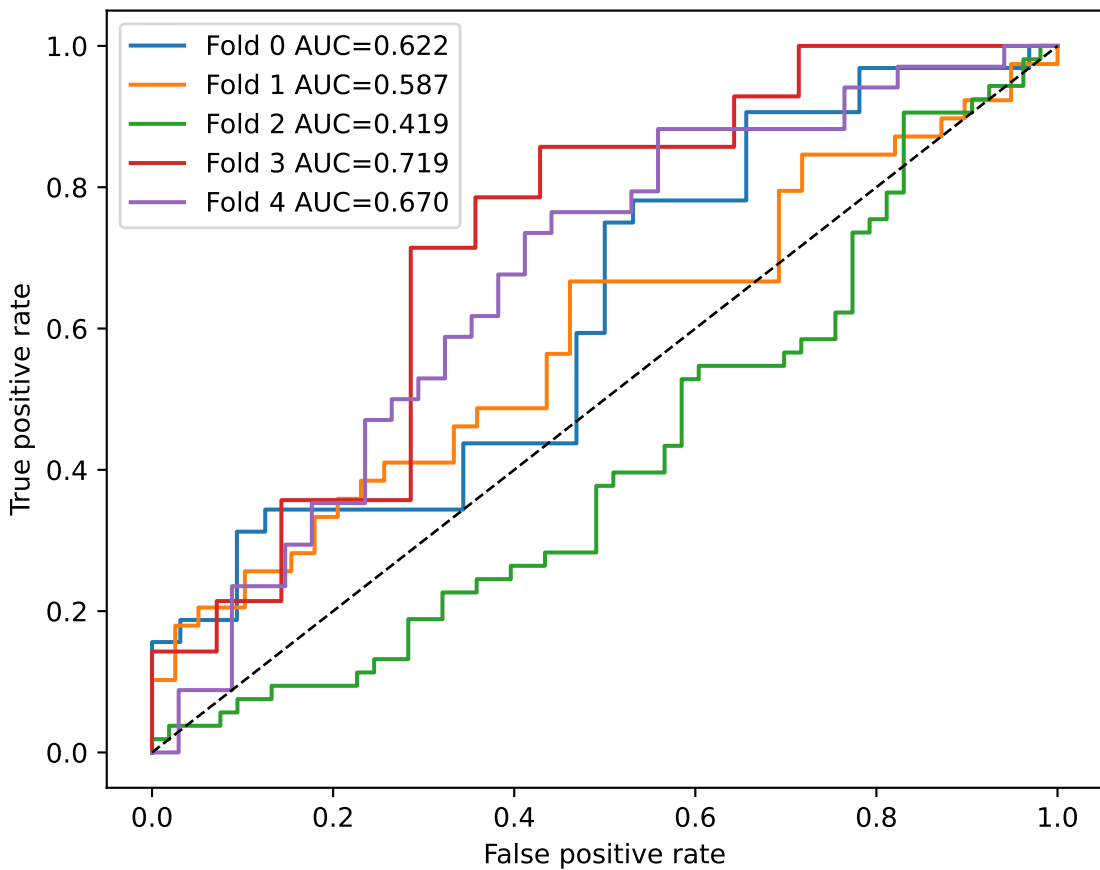
ROC curves, mean AUC=0.604
