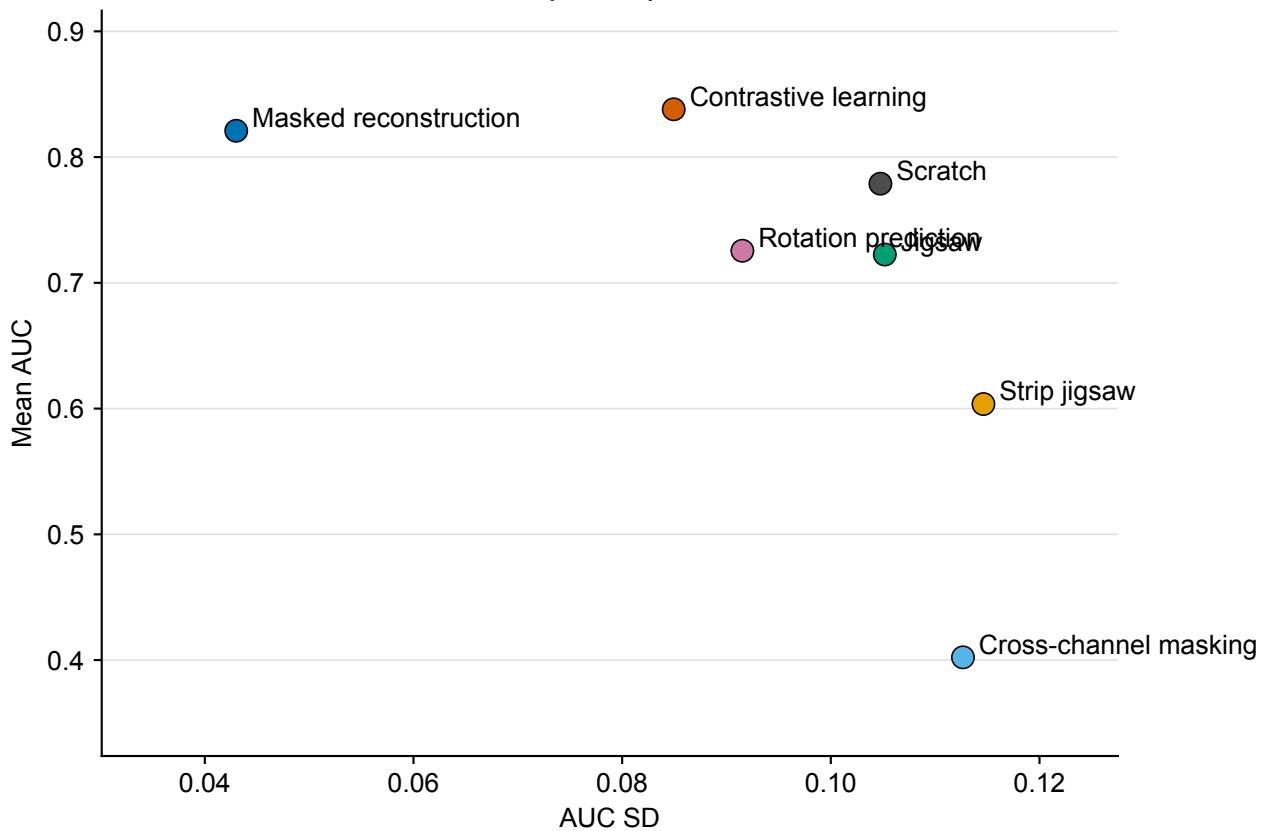
Accuracy-stability trade-off
