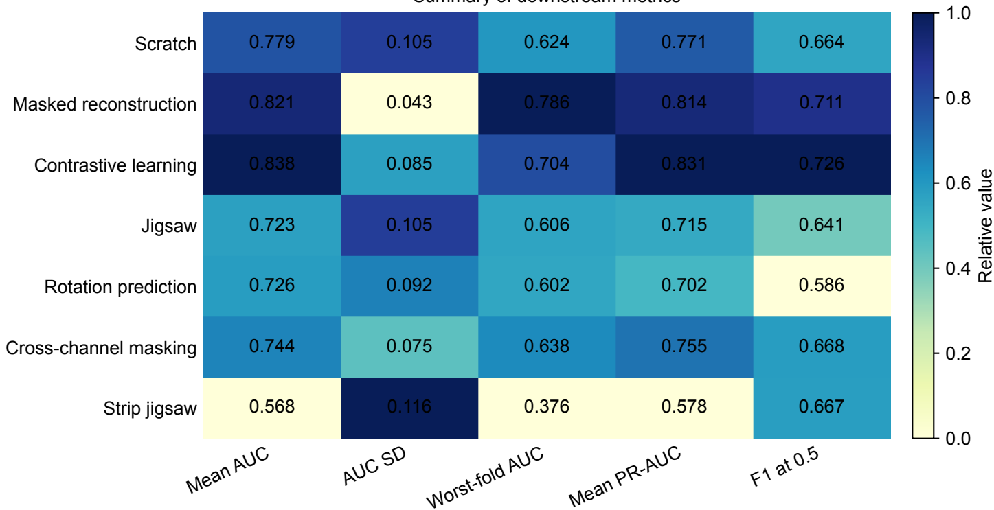
Summary of downstream metrics
