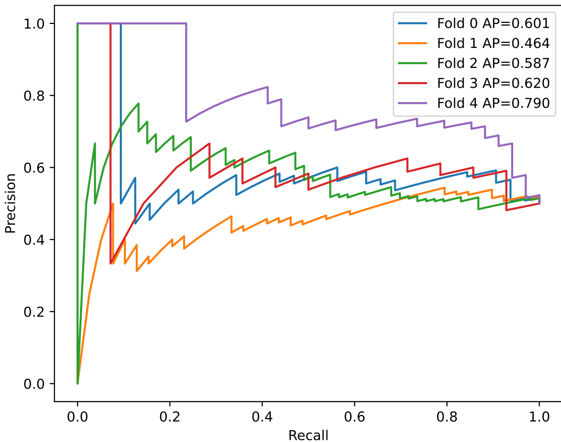
PR curves, mean AP=0.612
