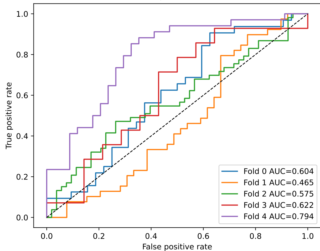
ROC curves, mean AUC=0.612
