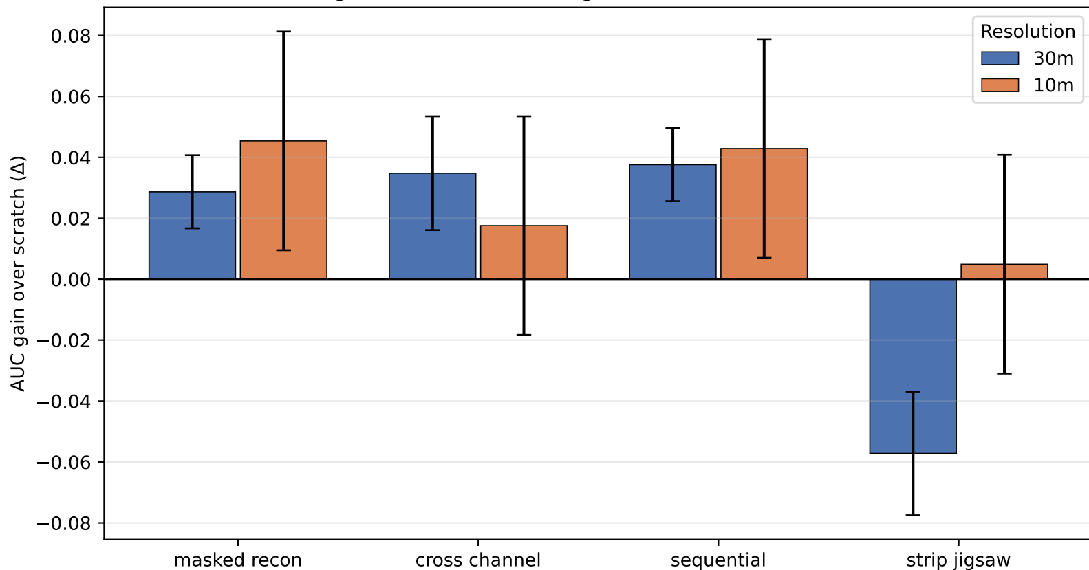
Does each SSL task beat scratch? (bar clearing its error bar = REAL gain; error bar = seed-to-seed noise)
