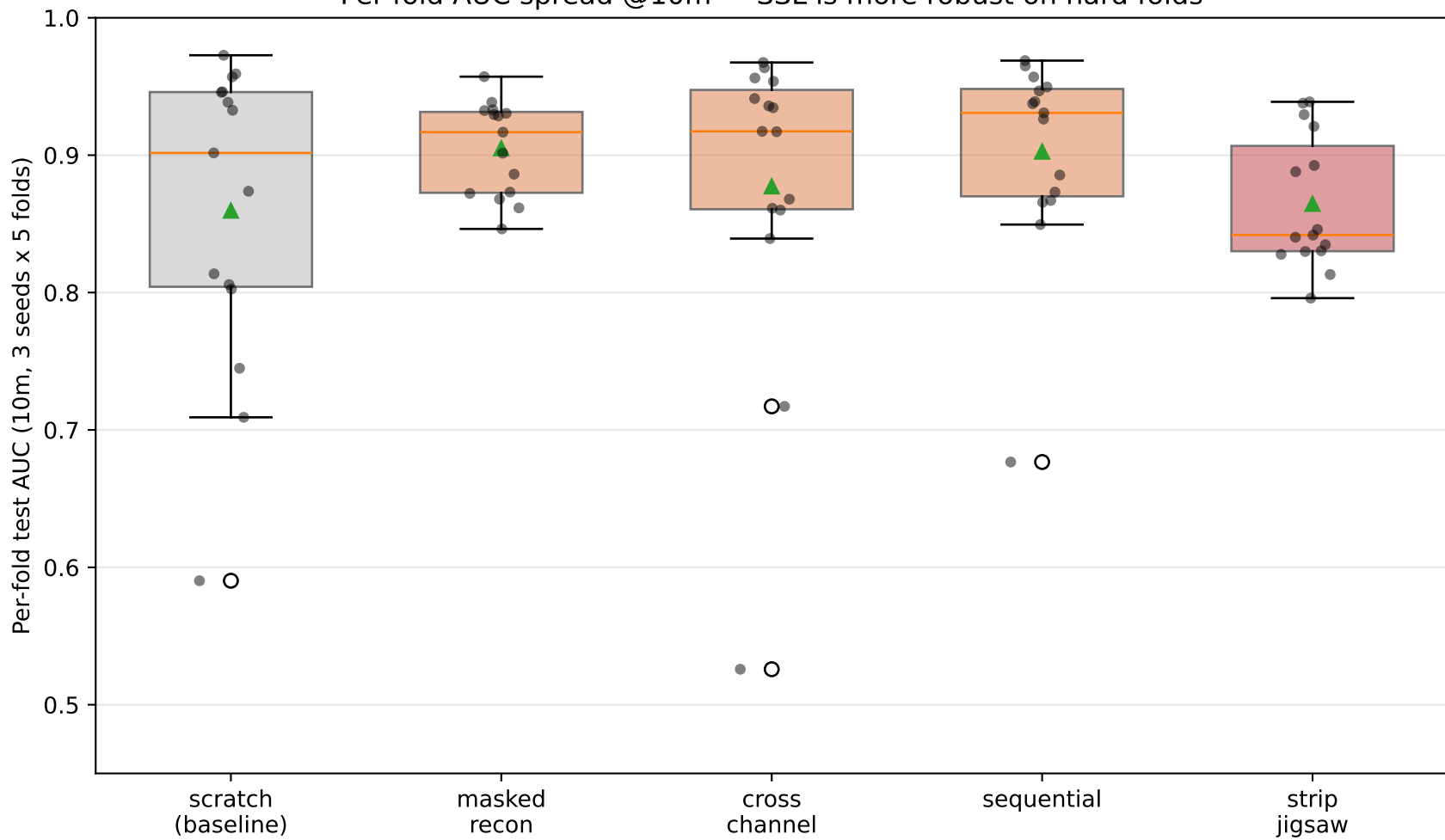
Per-fold AUC spread @10m — SSL is more robust on hard folds
