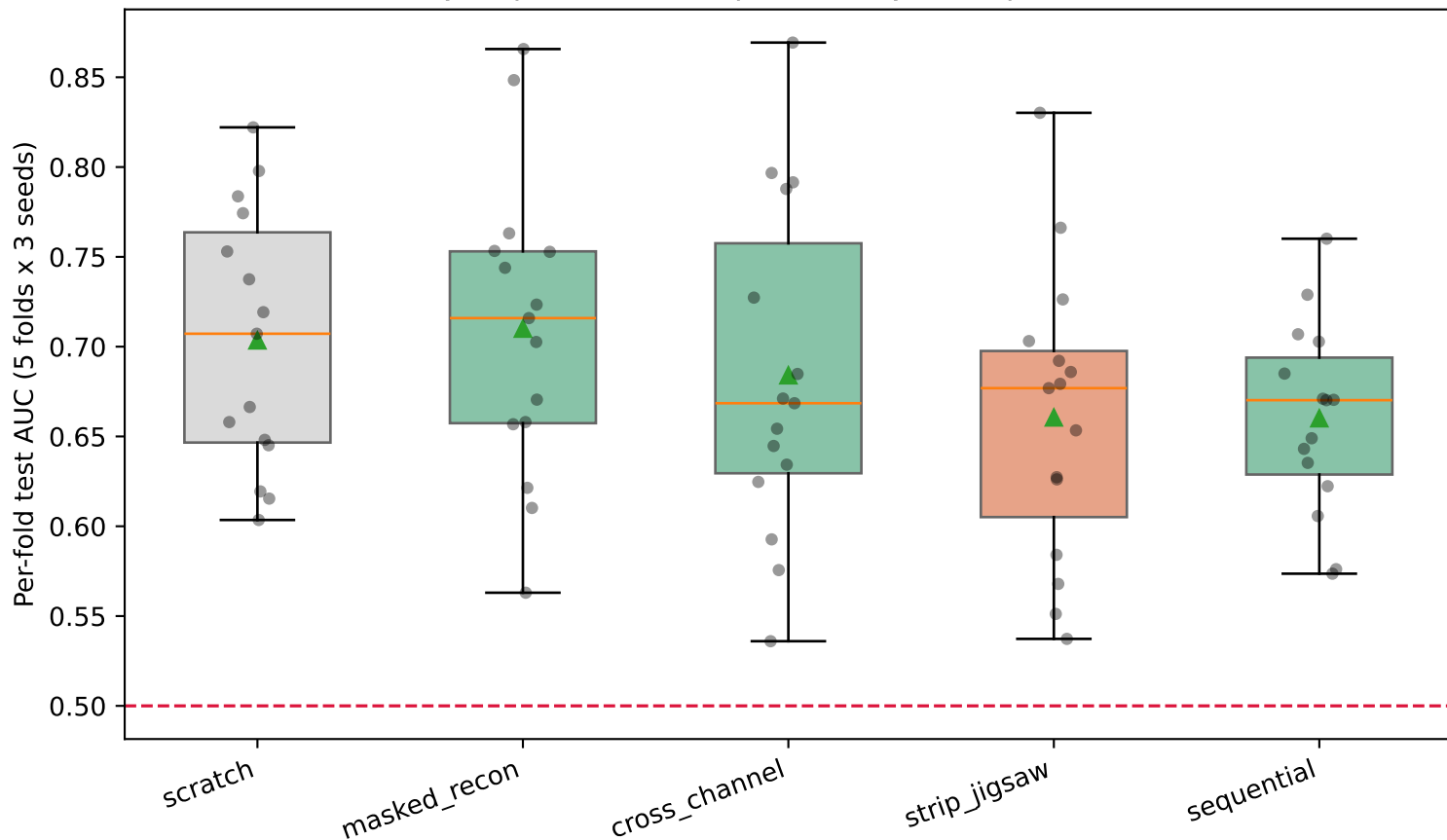
Kentucky — per-fold AUC spread (why we report multi-seed)
