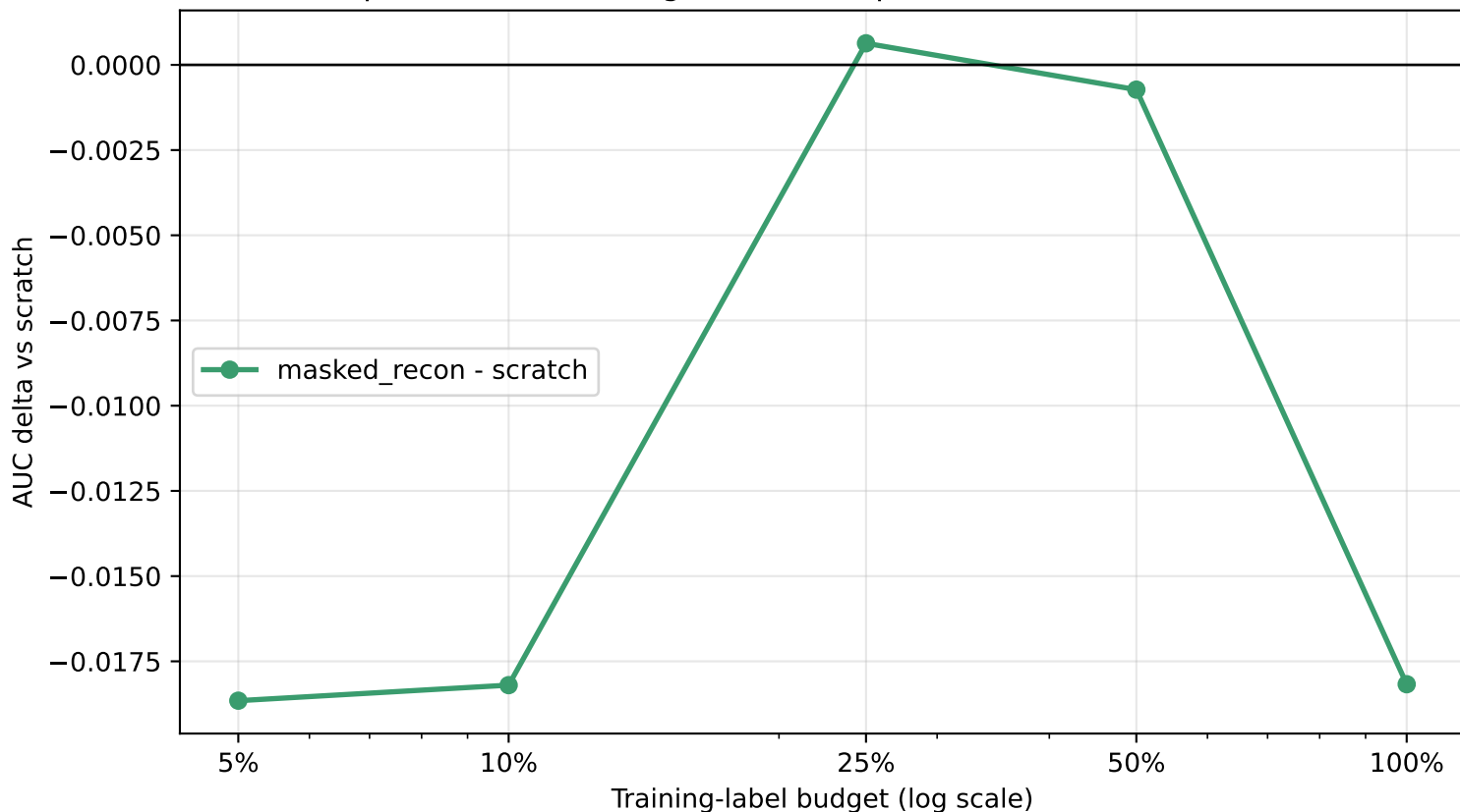
Kentucky — SSL minus scratch vs label budget (positive at low budget = SSL helps when labels are scarce)
