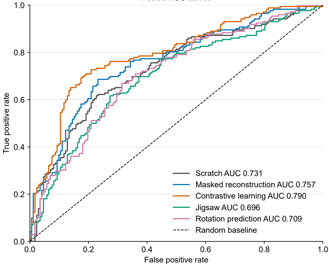
Pooled ROC curves
