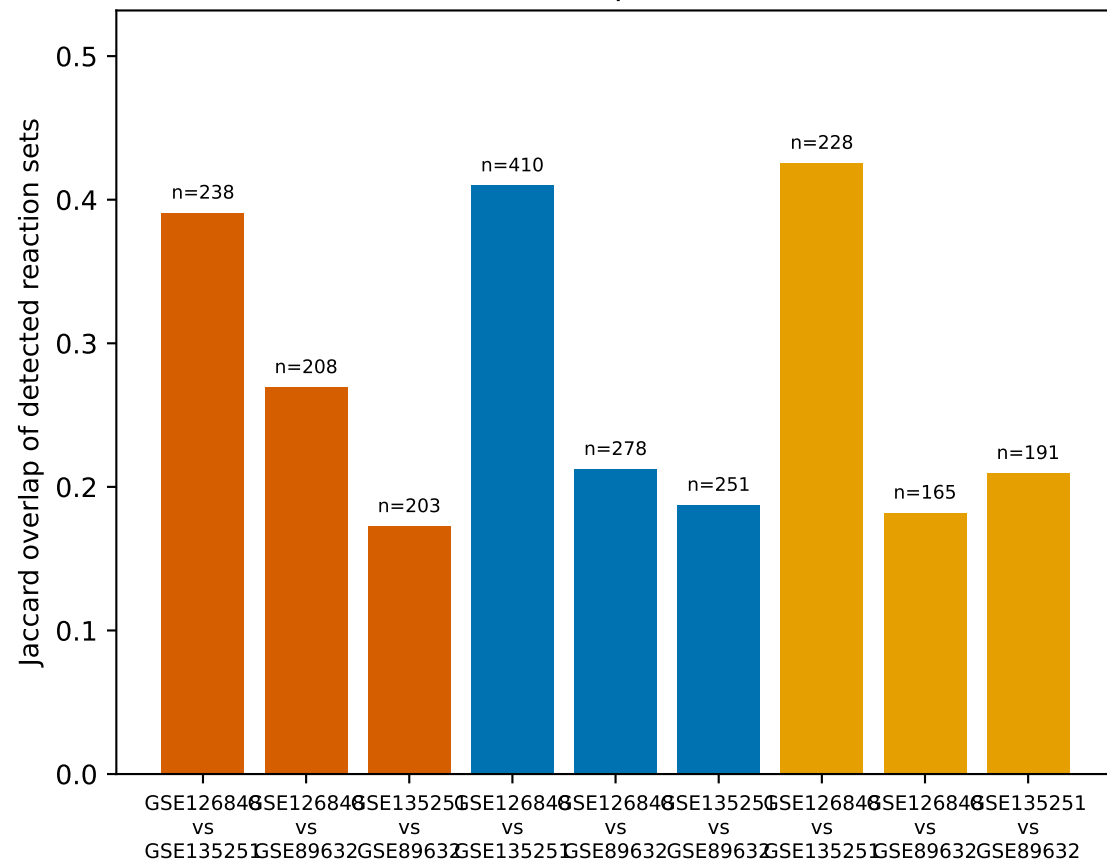
D2. Detected-set overlap (both/either detected)
