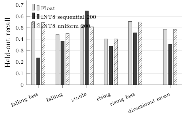
Figure 3: Per-class held-out recall, mean over five seeds (and three draws for the uniform arm). The sequential-200 calibration collapses falling_fast and inflates stable ; a uniform random selection of the same size restores the float profile.
