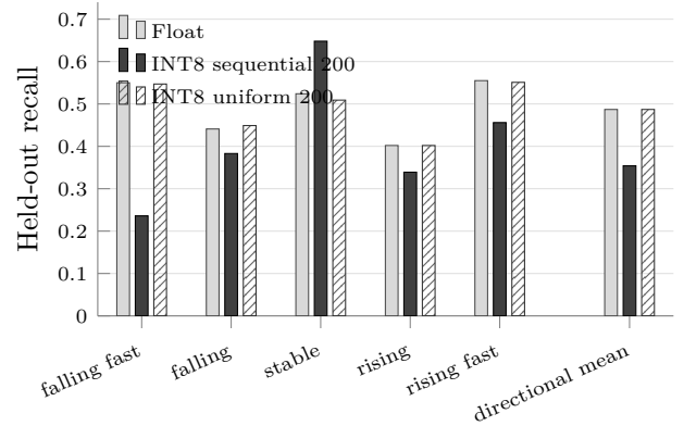
Figure 3: Per-class held-out recall, mean over five seeds (and three draws for the uniform arm). The sequential-200 calibration collapses falling_fast and inflates stable ; a uniform random selection of the same size restores the float profile.
