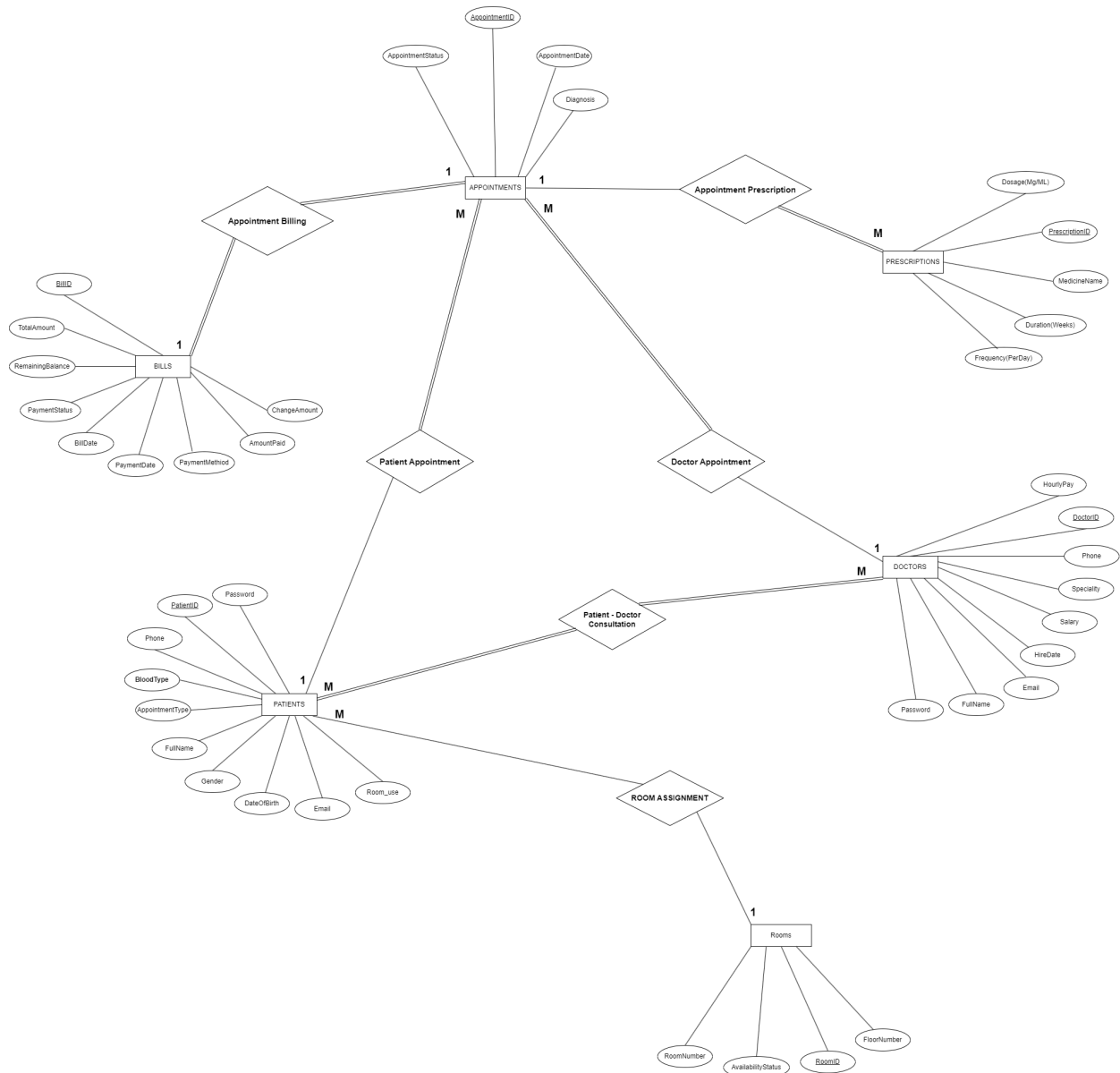
Figure 1 — SmartClinic Entity-Relationship Diagram
