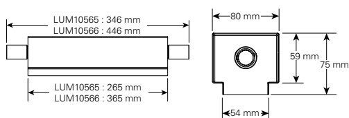
Concrete box
