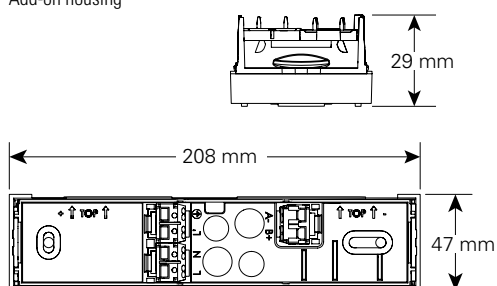
Add-on housing
