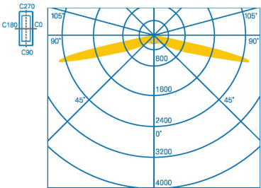
Ceiling mounting, Escape Route, LowBay
