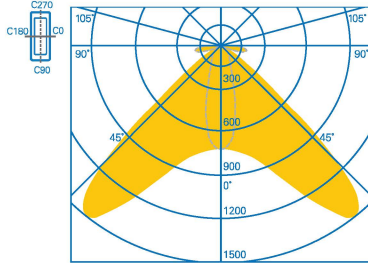
Ceiling mounting, Escape Route, HiBay
