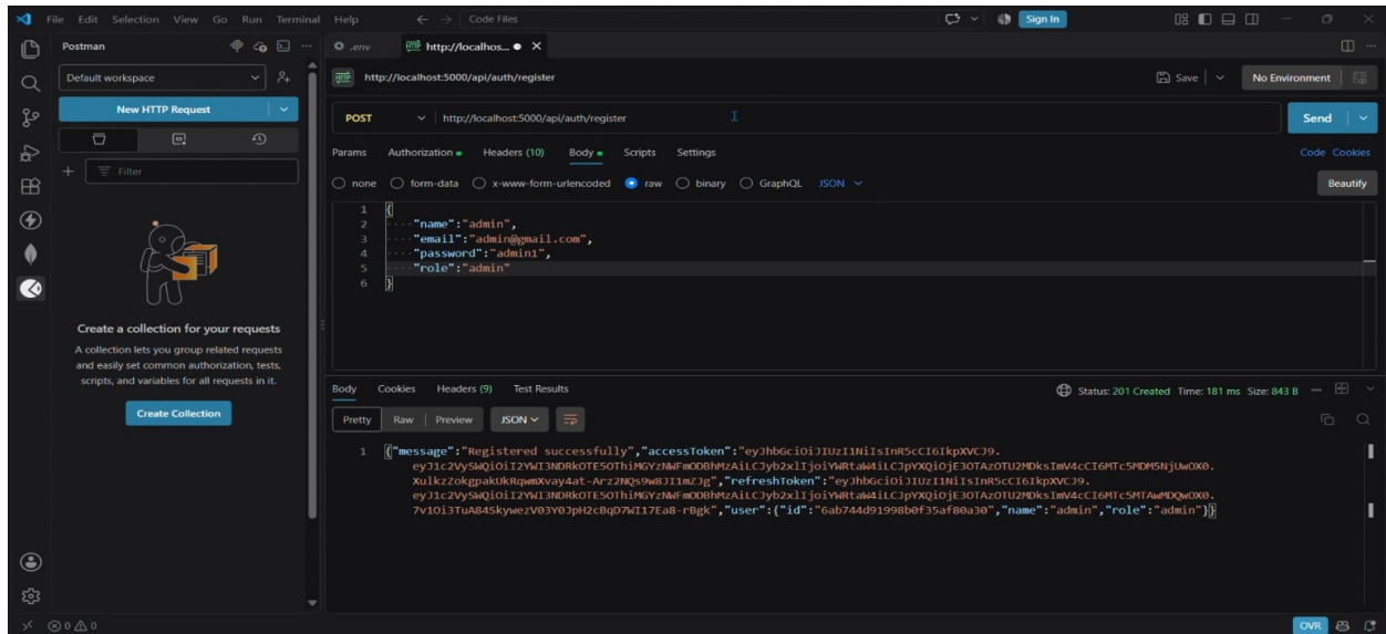
Figure 6.3: Administrator registration – HTTP 201 Created.
