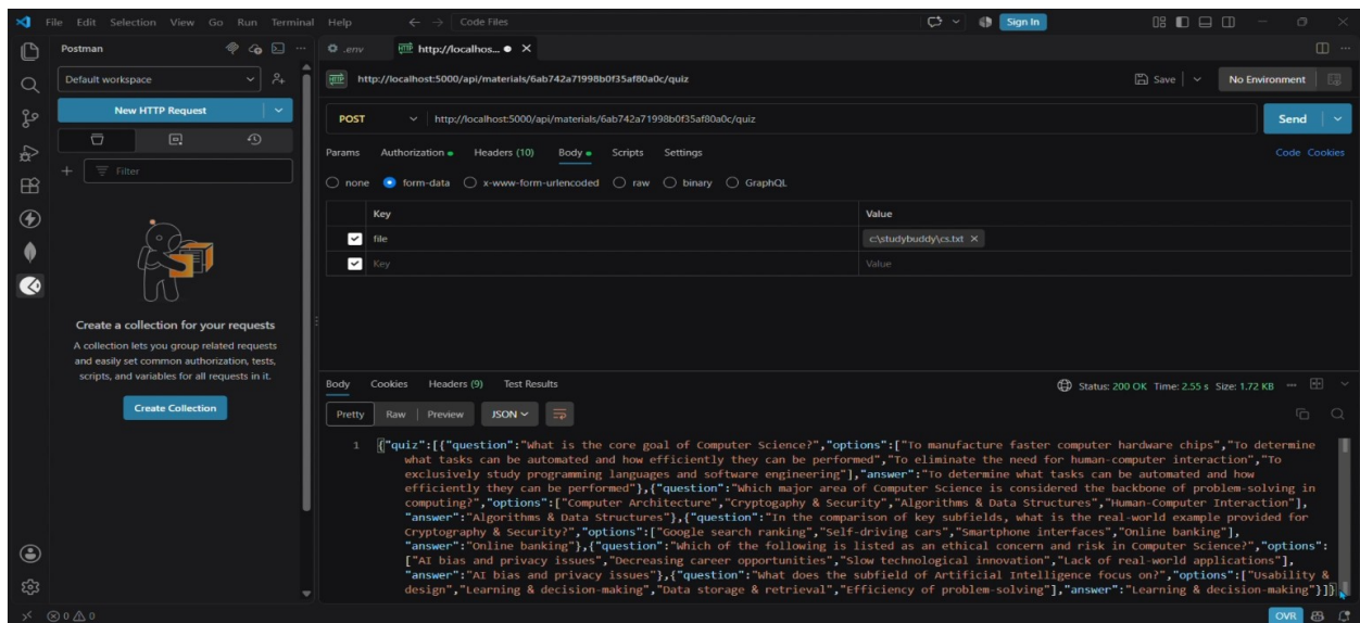
Figure 6.7: Quiz generation – HTTP 200 OK.
