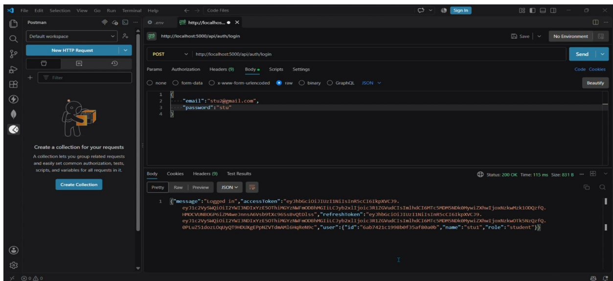
Figure 6.2: Student login – HTTP 200 OK.
