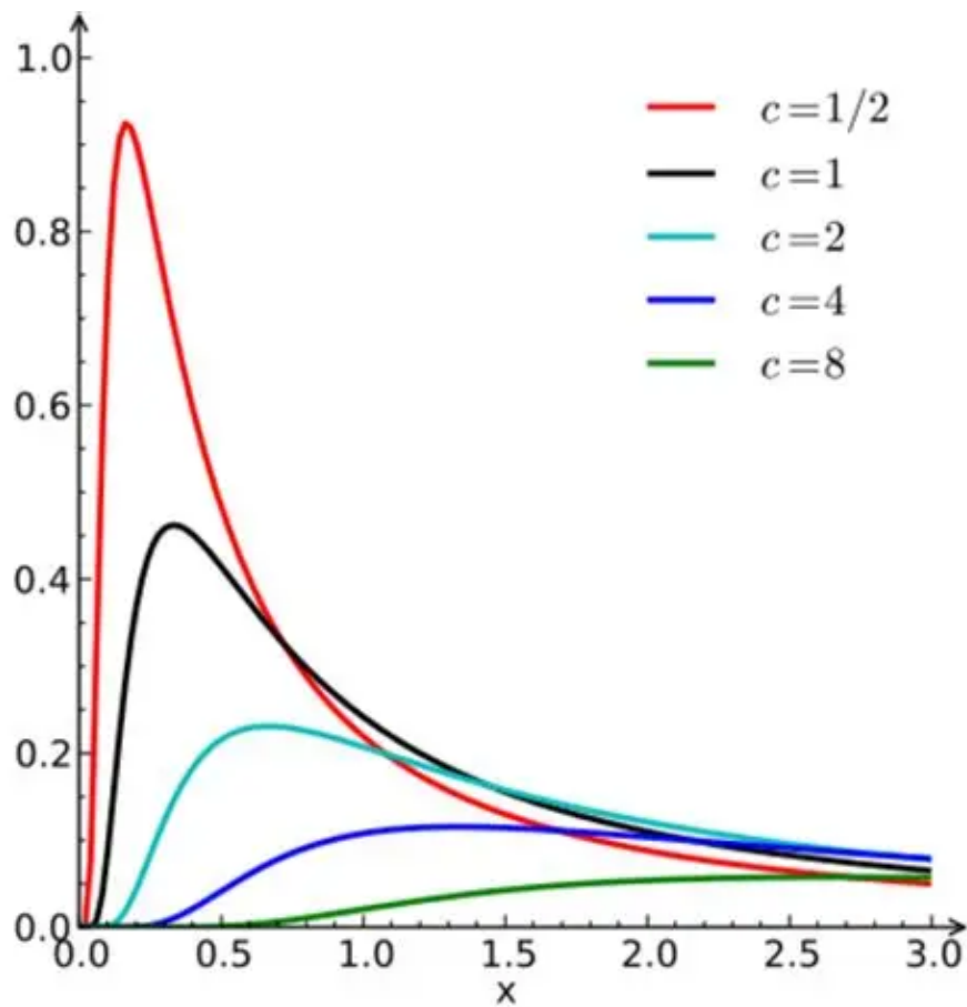
Figure 3.1 – Lévy PDF
