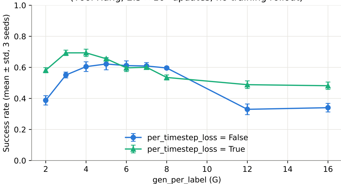
Drift Policy: success rate vs. G , 3-seed confirmatory sweep (Tool Hang, 2.5 \times 10^5 updates, no training rollout)
