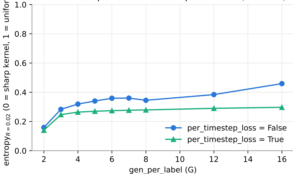
Attraction/repulsion kernel sharpness vs. G ( R = 0.02 )
