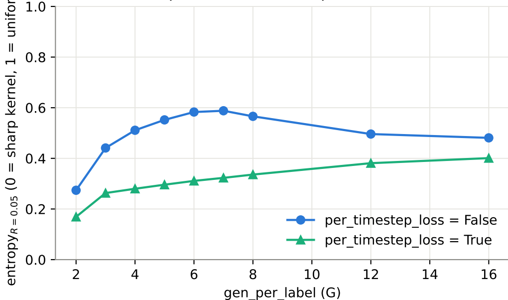
Attraction/repulsion kernel sharpness vs. G ( R = 0.05 )
