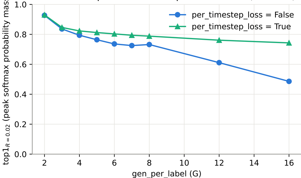
Attraction/repulsion kernel top-1 mass vs. G ( R = 0.02 )
