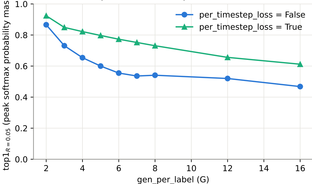
Attraction/repulsion kernel top-1 mass vs. G ( R = 0.05 )
