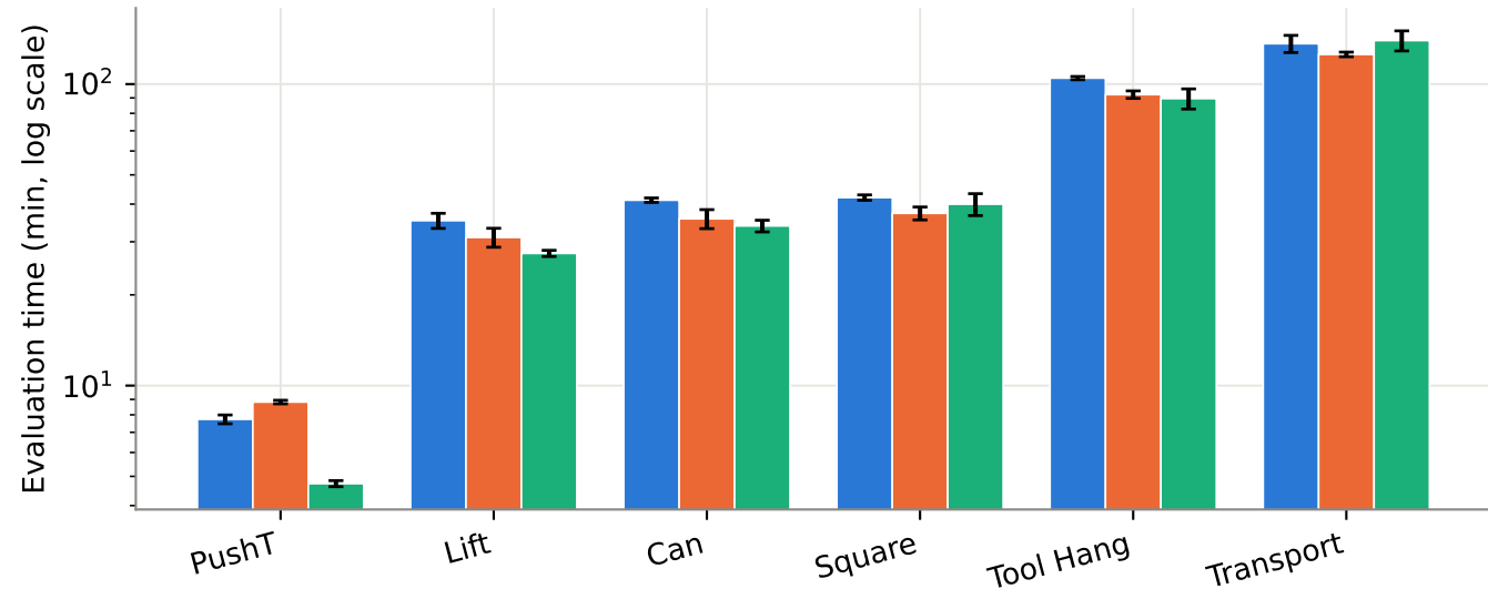
Diffusion Policy Flow Policy Drift Policy Full-rollout evaluation wall-clock time by task and method
