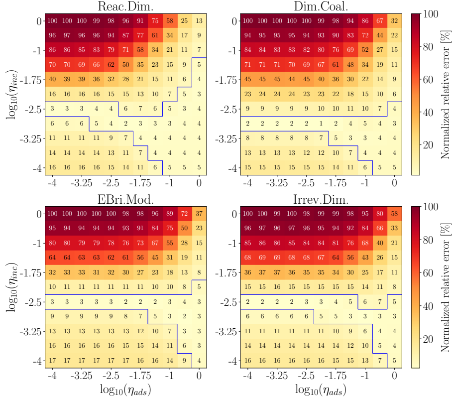
Figure 4.3: The relative error of CY normalized by the maximum value at t = 1.5 ms for 5% \text{CH}_4 -Ar obtained using Caltech mechanism and all PAH growth models. Each cell is annotated with its corresponding normalized relative error expressed in percent.
