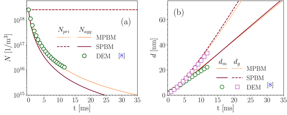
Figure 3.3: The number concentration of agglomerates and primary particles (a), and mobility and gyration diameters (b) obtained by Omnisoot using MPBM and SPBM in the free-molecular regime, which are in close agreement with the DEM results [8] indicating the validity of the coagulation sub-models.
