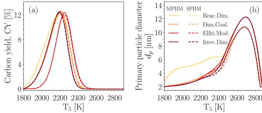
Figure A.1: The comparison of CY (a) and primary particle diameter, d_p , at t = 1.5 ms obtained using MPBM and SPBM models for the case optimized using equal adjustment factors to minimize the prediction error.
