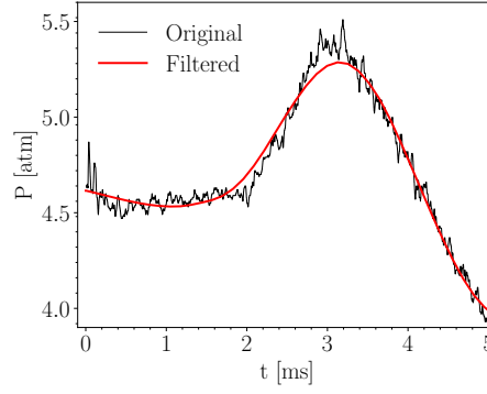
Figure 3.7: The pressure time history (black line) measured by the Stanford group for pyrolysis of 5%CH 4 at T_5 = 2355 K and P_5 = 4.64 atm, and filtered (red line) with reduced fluctuations used to specify the pressure of the reactor
