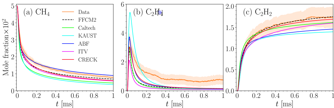
Figure 4.1: The mole fraction of \text{CH}_4 (a), \text{C}_2\text{H}_4 and \text{C}_2\text{H}_2 (c) during pyrolysis of 5% \text{CH}_4 -Ar predicted using different reaction mechanisms and compared with measurements [9].
