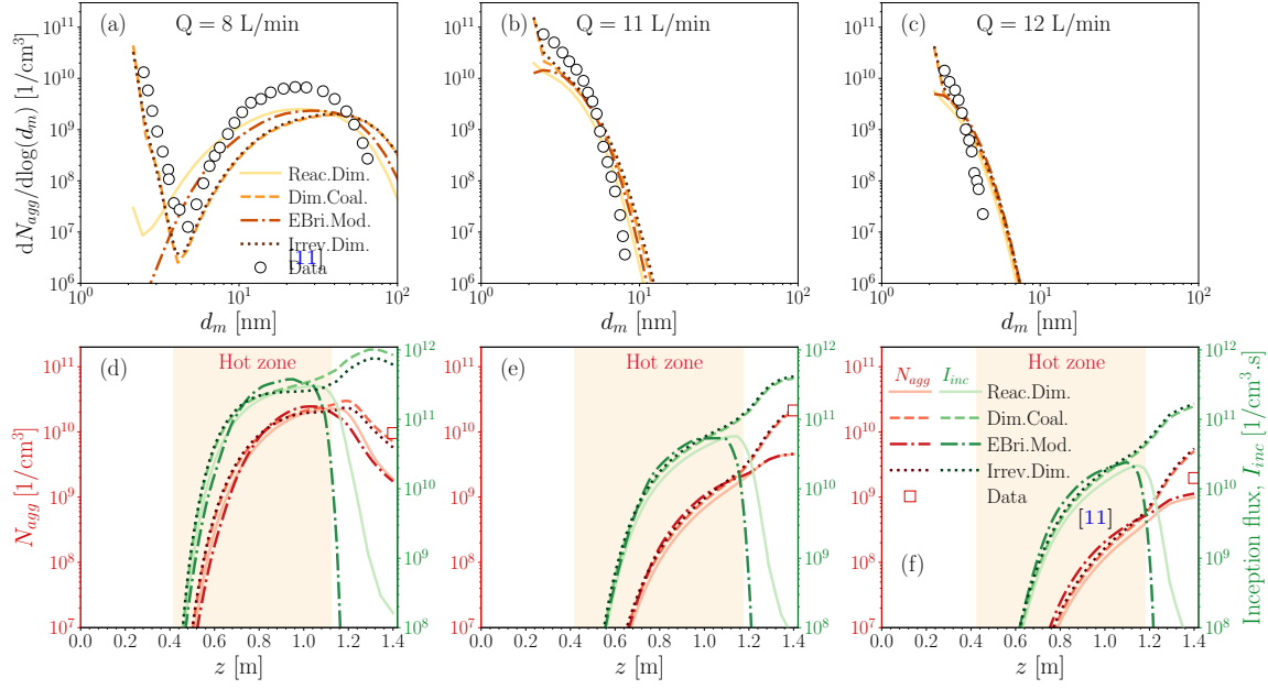
Figure 4.11: The particle size distribution at the end of PFR, and the total number of agglomerates, N_{agg} , and inception flux, I_{inc} along the PFR for Q = 8 (a, d), 11 (b, e), and 12 L/min (c, f) obtained using KAUST mechanism, SPBM and different inception models calibrated to match the predictions with measurement [11].
