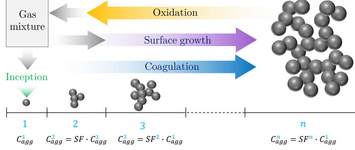
Figure 2.5: The illustration of sections in SPBM. The mass of sections grows progressively by the scale factor of SF. Inception introduces new particles to the first section that propagate to the upper section via coagulation and surface growth and return to lower sections by oxidation. Carbon and hydrogen pass from gas to solid phase through inception and surface growth and goes back via oxidation.
