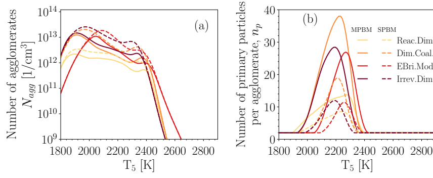
Figure A.2: The temperature dependence of total number of agglomerates, N_{agg} (a), number of primary particles per agglomerate, n_p (b), at t = 1.5 ms obtained using MPBM and SPBM models for the case optimized using equal adjustment factors to minimize the prediction error.
