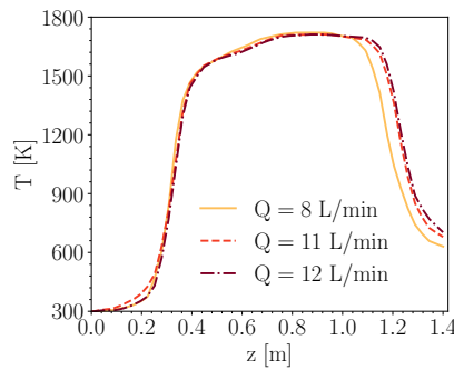
Figure 4.10: The centerline temperature along the reactor for Q = 8, 11 , and 12 L/min interpolated from the thermocouple measurements [11].
