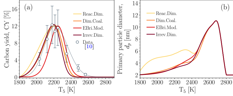
Figure 4.6: The CY (a) and primary particle diameter, d_p , (b) at t = 1.5 ms during the pyrolysis of 5% \text{CH}_4 -Ar obtained using equal adjustment factors to minimize the prediction error with extinction measurements [10]. The dashed line was added to show the trend in the measurements.
