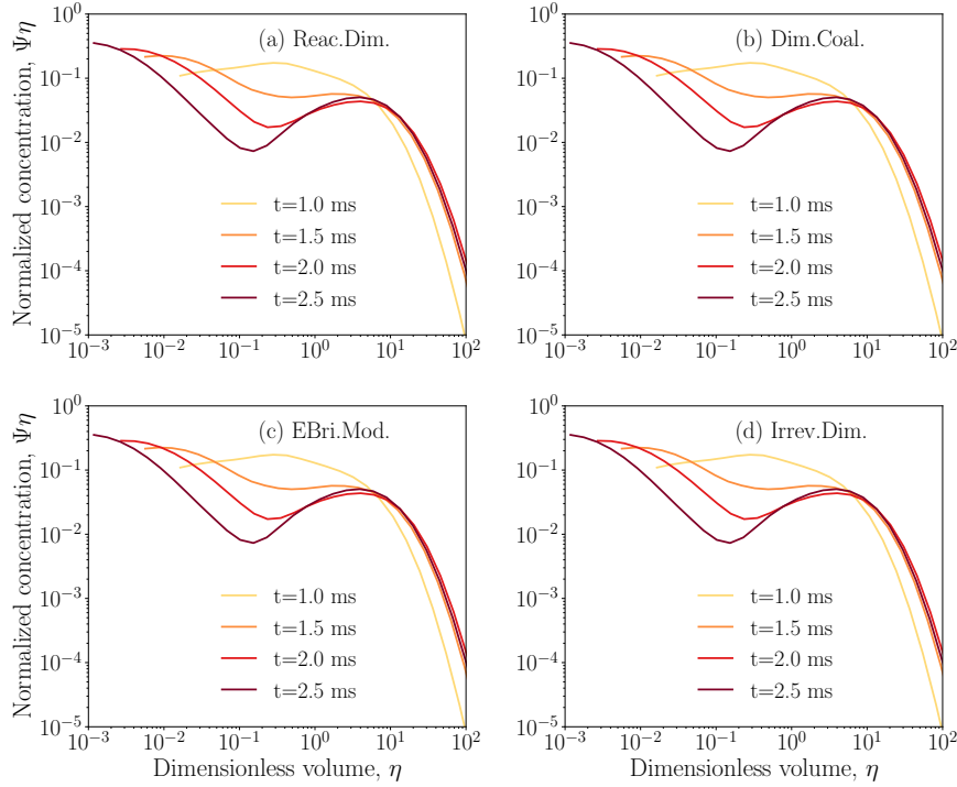
Figure A.3: The non-dimensional particle size distribution during 5%CH 4 -Ar at T_5 = 2200 K that evolves from 1 ms to 2.5 ms indicating SPSP is not attained yet.
