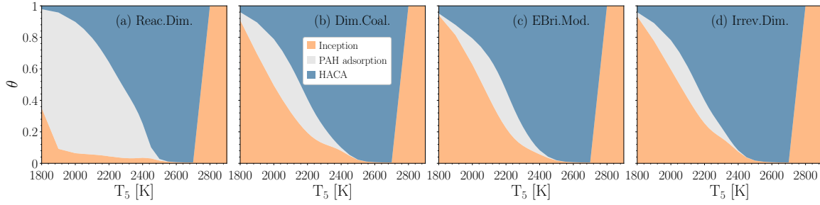
Figure 4.7: The variation of \theta , defined as soot carbon mass from inception, PAH adsorption and HACA normalized by total soot carbon mass at t = 1.5 ms during the pyrolysis of 5% \text{CH}_4 -Ar.
