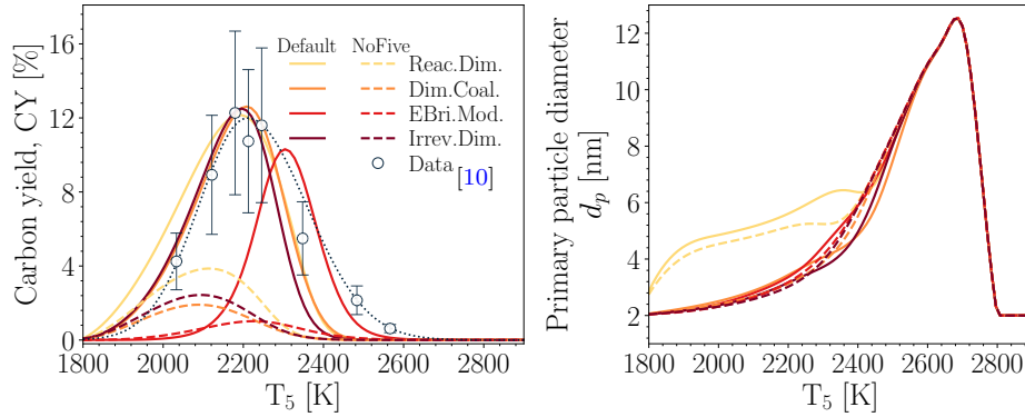
Figure 4.5: The soot carbon yield, CY, at t = 1.5 ms (a) and primary particle diameter, d_p (b) obtained using the default soot precursors (denoted by solid line and labeled as “Default”) compared with the same results when five-membered ring PAHs excluded from soot precursors (denoted by dashed line and labeled as “NoFive”). Both cases were obtained using Caltech mechanism and the same equal adjustment factors. The black dashed line was added to show the trend in the measurements [10].
