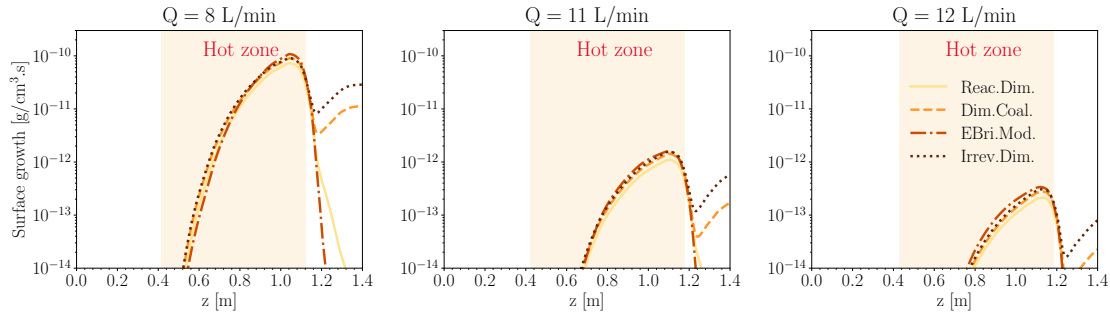
Figure A.5: The surface growth by HACA and PAH adsorption combined along the PFR for Q = 8 (a), 11 (b), and 12 L/min (c) obtained using KAUST mechanism, SPBM and different inception models. The yellow area represents the hot zone ( T > 0.9T_{\max} ).
