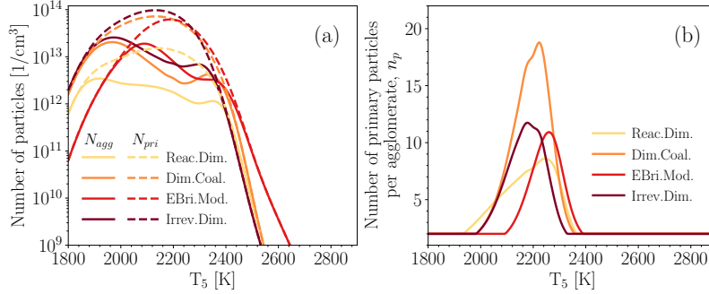
Figure 4.8: The temperature dependence of total number of agglomerates, N_{agg} (a), number of primary particles per agglomerate, n_p (b) at t = 1.5 ms during the pyrolysis of 5% \text{CH}_4 -Ar.
