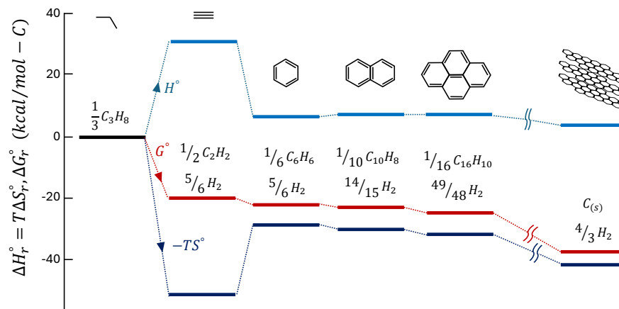
Figure 1.2: Standard enthalpy ( \Delta H ) and entropy ( T\Delta S ) contributions to Gibbs function of reaction \Delta G at 1600 K for carbon formation from propane(reprinted from Ref. [4])
