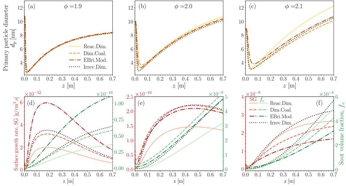
Figure 4.14: The primary particle diameter, d_p , the total surface growth rate by HACA and PAH adsorption, and the soot volume fraction, f_v along the PFR for \phi = 1.9 (a, d), 2.0 (b, e), and 2.1 (c, f) obtained using KAUST mechanism, SPBM and different inception models calibrated to match the predictions with the PSD measurements [137].
