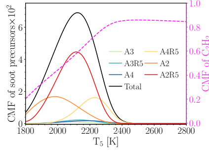
Figure 4.4: The bell-shaped temperature profile of carbon mass fraction of soot precursors (A2 and larger) combined and C_2H_2 at t = 1.5 ms during pyrolysis of 5% CH_4 -Ar obtained using Caltech mechanism without considering soot.
