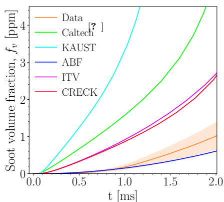
Figure 4.2: The maximum soot volume fraction predicted using Irreversible Dimerization and different reaction mechanisms during pyrolysis of 5% \text{CH}_4 -Ar was compared with measurements [9]. The shaded area represents the uncertainty in the reported experimental data.
