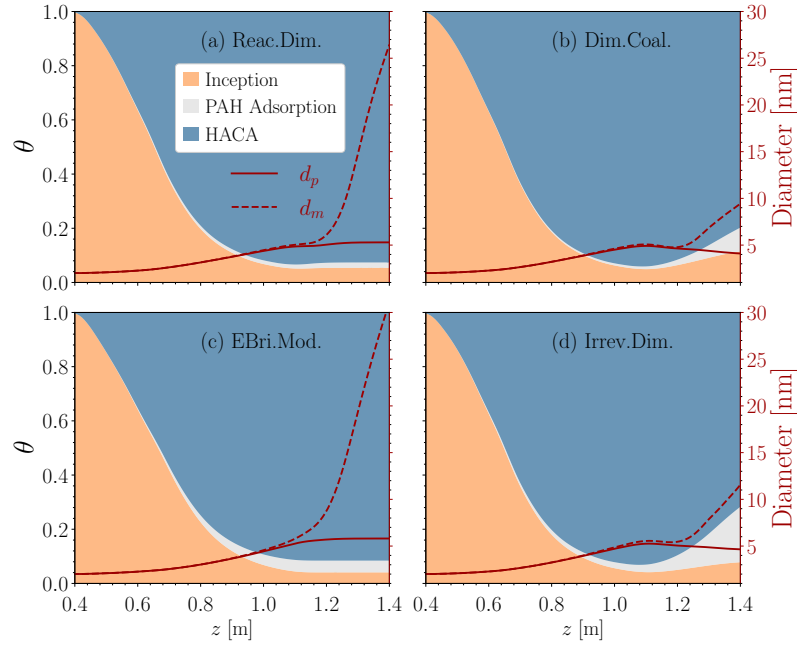
Figure 4.12: The variation of \theta , defined as soot carbon mass from inception, PAH adsorption and HACA normalized by total soot carbon mass for Q = 8 L/min along with d_p and d_m obtained using KAUST mechanism, SPBM and different inception models.
