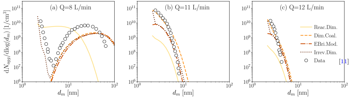
Figure A.4: The particle size distribution at the end of PFR for Q = 8 (a), 11 (b), and 12 L/min (c) obtained using Caltech mechanism, SPBM and different inception models calibrated to match the predictions with measurement [11].
