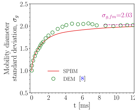
Figure 3.5: Standard deviation of the mobility diameter, \sigma_g , in the free-molecular regime obtained by SPBM is in close agreement with DEM results [8].
