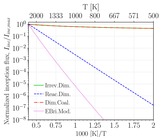
Figure 2.6: The temperature dependence of inception flux, I_{inc} , predicted using various PAH growth models. I_{inc} of each model is normalized with its maximum to facilitate the comparison.
