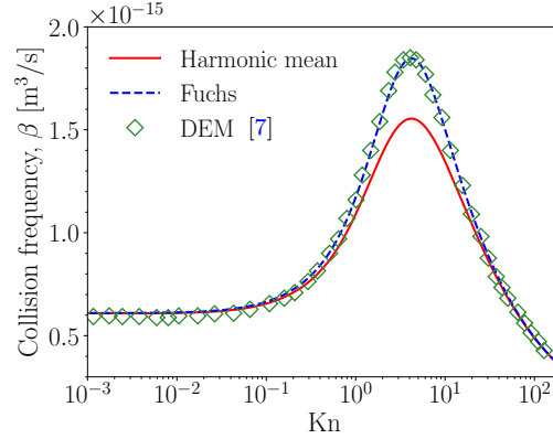
Figure 3.1: The comparison of collision frequency, \beta , obtained by Omnisoot using harmonic mean (red solid line) and Fuchs interpolations (blue dashed line) with DEM results (symbols) [7].
