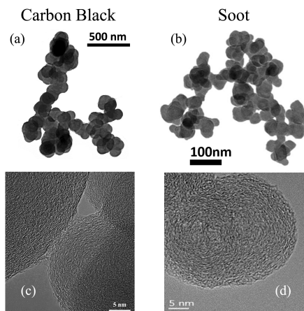
Figure 1.1: The TEM images of Carbon black (a & c) [1] and soot (b & d) [2, 3] that shows soot and CB has similar morphology and structure
