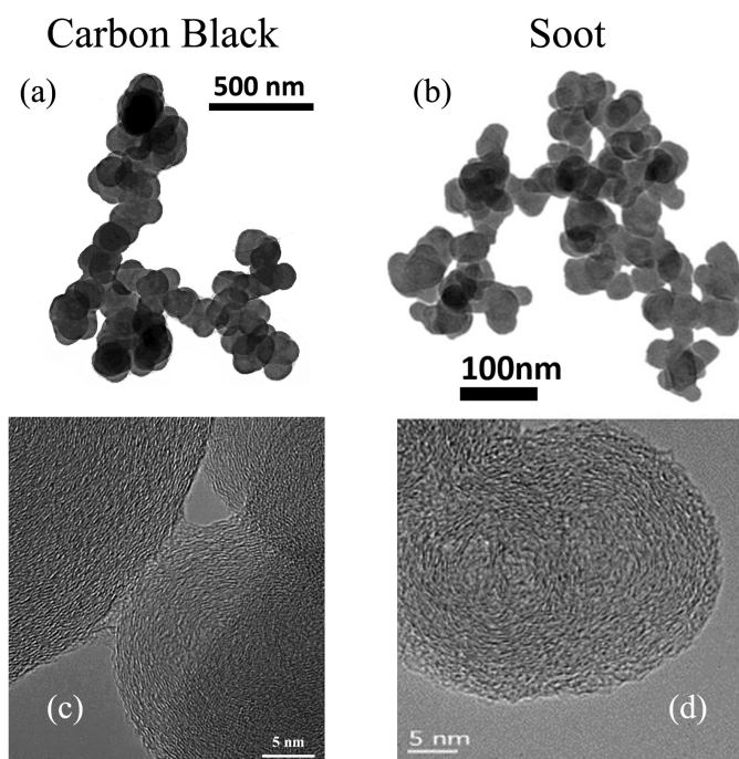
Fig. 1.1 The TEM images of Carbon black (a & c) [12] and soot (b & d) [13, 14] that shows soot and CB has similar morphology and nanostructure.
