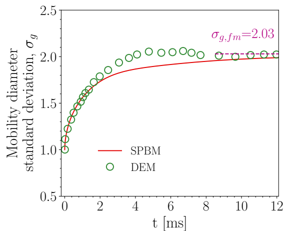
Fig. 3.5 Standard deviation of the mobility diameter, \sigma_g , in the free-molecular regime obtained by SPBM is in close agreement with DEM results [147].
