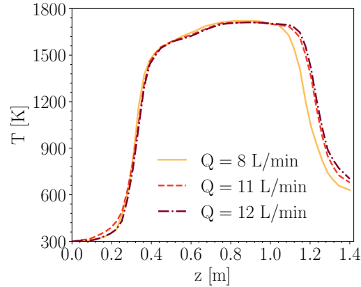
Fig. 4.10 The centerline temperature along the reactor for Q = 8, 11 , and 12 L/min interpolated from the thermocouple measurements [177].
