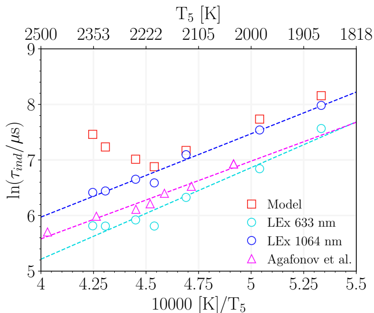
Fig. 4.30 The predicted soot induction time, \tau_{ind} , compared with light extinction measurements at 633 nm and 1064 nm, and with the data from Agafonov et al. [216]. The dashed line is the Arrhenius fit to the measurements.
