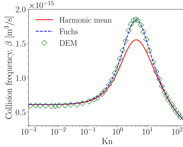
Fig. 3.1 The comparison of collision frequency, \beta , obtained by Omnisoot using harmonic mean (red solid line) and Fuchs interpolations (blue dashed line) with DEM results (symbols) [162].
