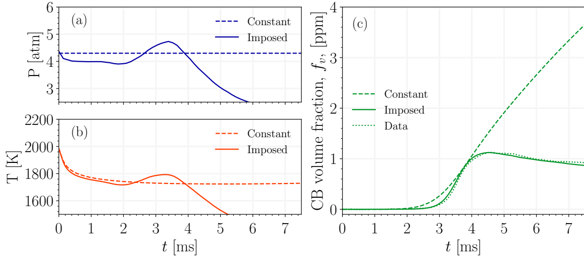
Fig. 4.16 The comparison of (a) pressure (b) temperature (c) CB volume fraction for simulations with constant and imposed pressure trace at T_5=1984 K.
