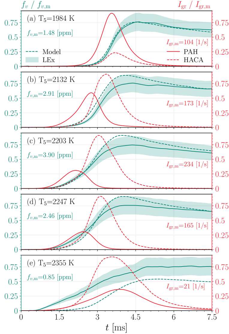
Fig. 4.19 The time histories of normalized CB volume fraction, f_v/f_{v,m} and normalized surface growth, I_{gr}/I_{gr,m} at various temperatures. The measurements are from light extinction at \lambda = 1064 nm with the shaded area representing the uncertainty from the variability in E(m) .
