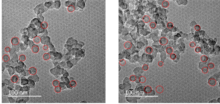
Fig. 4.15 Samples of TEM images collected for T_5=2203 K. Red circles represent the identified primary particles used to measure d_p .
