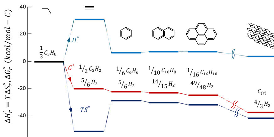
Fig. 1.2 Standard enthalpy ( \Delta H ) and entropy ( T\Delta S ) contributions to Gibbs function of reaction \Delta G at 1600 K for carbon formation from propane(reprinted from Ref. [182])
