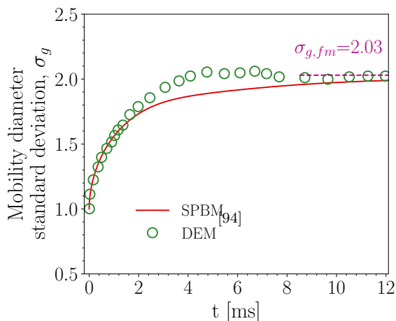
Fig. 3.5 Standard deviation of the mobility diameter, \sigma_g , in the free-molecular regime obtained by SPBM is in close agreement with DEM results [94].
