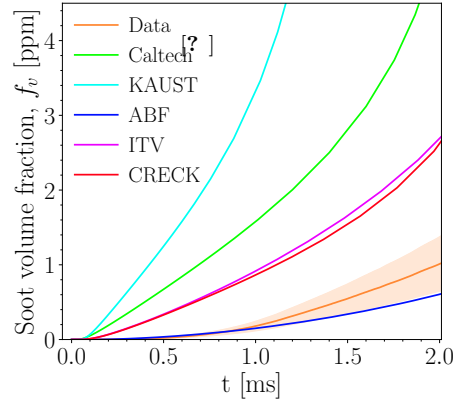
Fig. 4.2 The maximum soot volume fraction predicted using Irreversible Dimerization and different reaction mechanisms during pyrolysis of 5% \text{CH}_4 -Ar was compared with measurements [58]. The shaded area represents the uncertainty in the reported experimental data.
