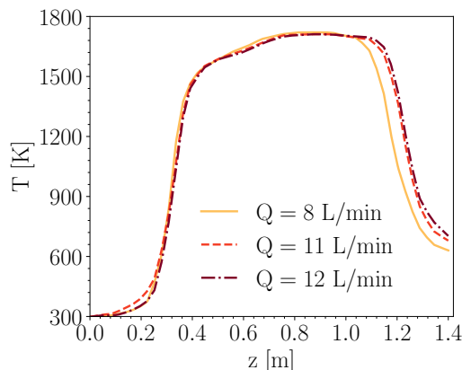
Fig. 4.10 The centerline temperature along the reactor for Q = 8, 11 , and 12 L/min interpolated from the thermocouple measurements [115].
