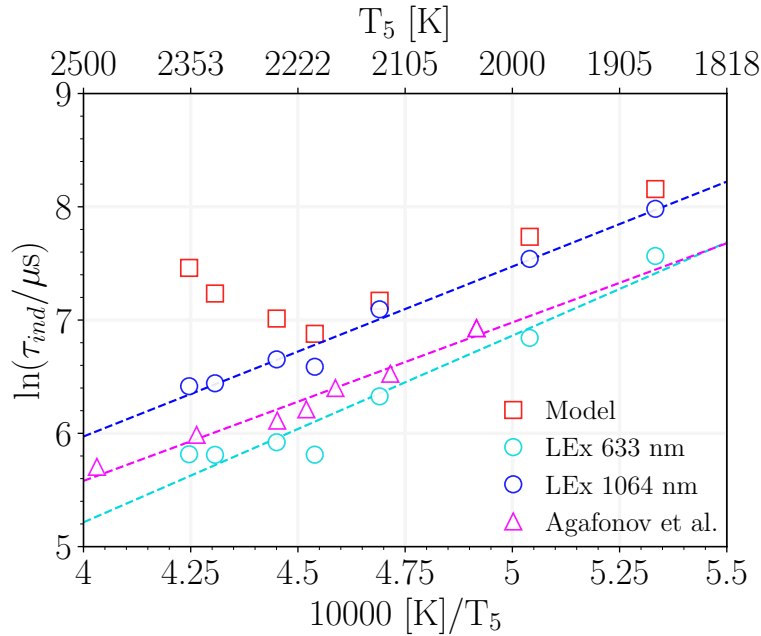
Fig. 4.21 The predicted CB induction time, \tau_{ind} , compared with light extinction measurements at 633 nm and 1064 nm, and with the data from Agafonov et al. [5]. The dashed line is the Arrhenius fit to the measurements.
