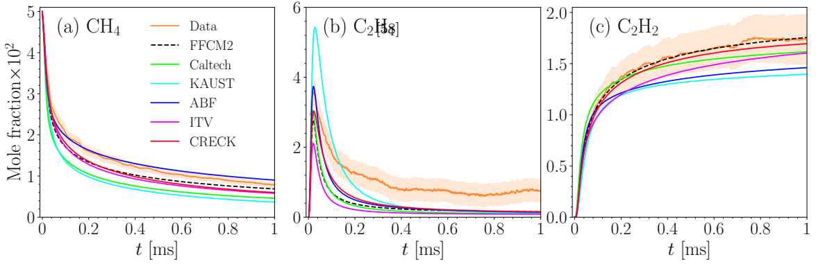
Fig. 4.1 The mole fraction of \text{CH}_4 (a), \text{C}_2\text{H}_4 and \text{C}_2\text{H}_2 (c) during pyrolysis of 5% \text{CH}_4 -Ar predicted using different reaction mechanisms and compared with measurements [58].
