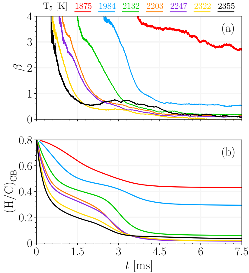
Fig. 4.24 The evolution of (a) maturity index, \beta , obtained from extinction measurements at 633 nm and 1064 nm, and (b) the predicted H/C ratio of CB particles at various T_5 .
