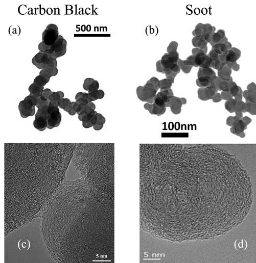
Fig. 1.1 The TEM images of Carbon black (a & c) [161] and soot (b & d) [175, 100] that shows soot and CB has similar morphology and structure
