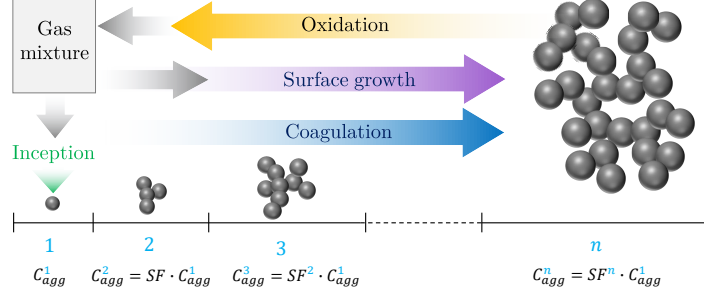
Fig. 2.5 The illustration of sections in SPBM. The mass of sections grows progressively by the scale factor of SF. Inception introduces new particles to the first section that propagate to the upper section via coagulation and surface growth and return to lower sections by oxidation. Carbon and hydrogen pass from gas to solid phase through inception and surface growth and goes back via oxidation.
