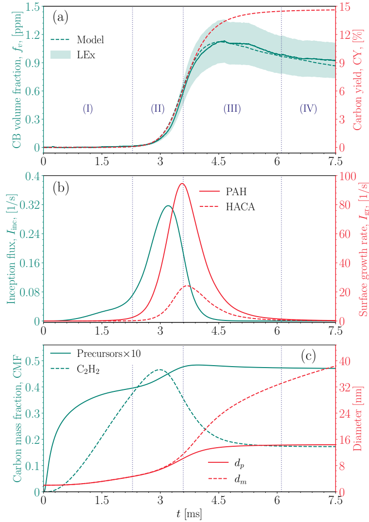
Fig. 4.18 The four stages of CB formation demonstrated at T_5 = 1984 K for (a) CB volume fraction, f_v , and carbon yield, CY (b) surface growth rate, I_{gr} , via HACA and PAH adsorption, and inception flux; (c) the carbon mass fraction, CMF, of C_2H_2 and CB precursors combined, and primary particle diameter, d_p , and mobility diameter d_m , of CB agglomerates. Panel (a) depicts the light extinction measurements at \lambda = 1064 nm with the shaded area representing the uncertainty from the variability in E(m) .
