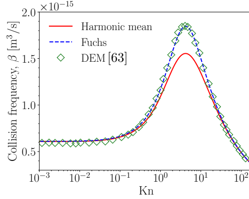
Fig. 3.1 The comparison of collision frequency, \beta , obtained by Omnisoot using harmonic mean (red solid line) and Fuchs interpolations (blue dashed line) with DEM results (symbols) [63].
