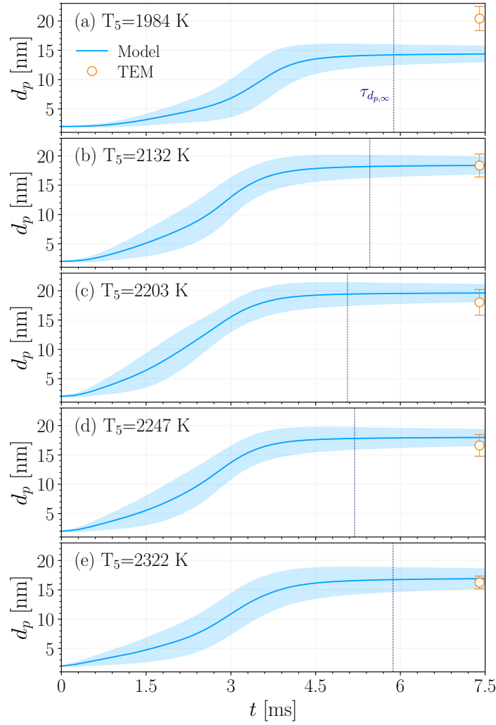
Fig. 4.20 The time histories of average primary particle diameter, d_p compared with TEM measurement. The shaded area, and error bar represents the d_p arithmetic standard deviation from the simulations and measurements, respectively. The dashed line specifies the time when d_p reaches 99% of its final value.
