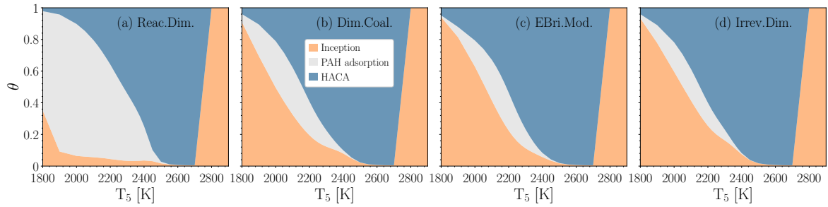
Fig. 4.7 The variation of \theta , defined as soot carbon mass from inception, PAH adsorption and HACA normalized by total soot carbon mass at t = 1.5 ms during the pyrolysis of 5% \text{CH}_4 -Ar.
