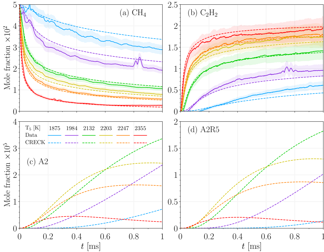
Fig. 4.17 The time history of (a) \text{CH}_4 and (b) \text{C}_2\text{H}_2 predicted using CRECK mechanisms in close agreement with the laser absorption measurements. The shaded area represents the uncertainty in the measurements.
