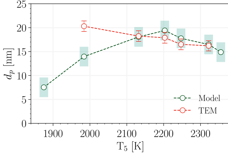
Fig. 4.23 The final primary particle diameter, d_p , from TEM measurements compared with the model predictions.
