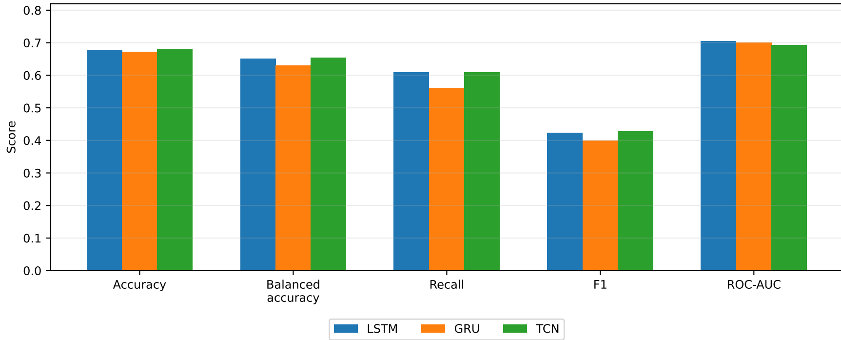
Best held-out test metrics by temporal representation
