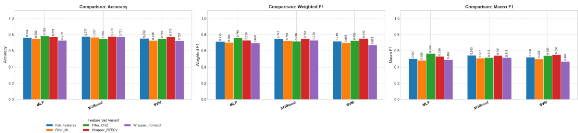
Algorithm vs. Feature Selection Comparison
