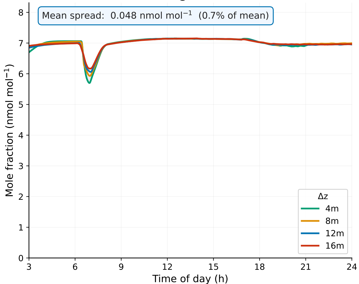
Reference height mole fraction
