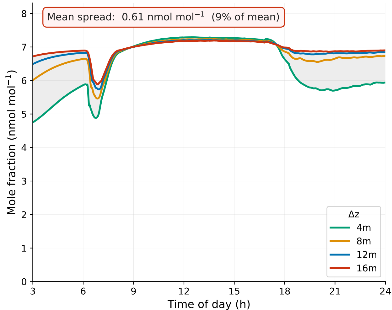
NH 3 surface mole fraction
