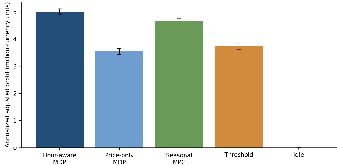
Synthetic performance over independently regenerated datasets
