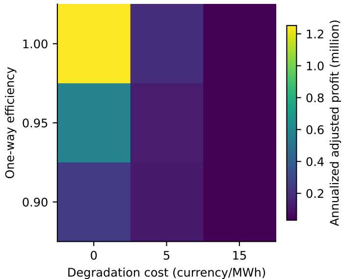
DK1 day-ahead block
