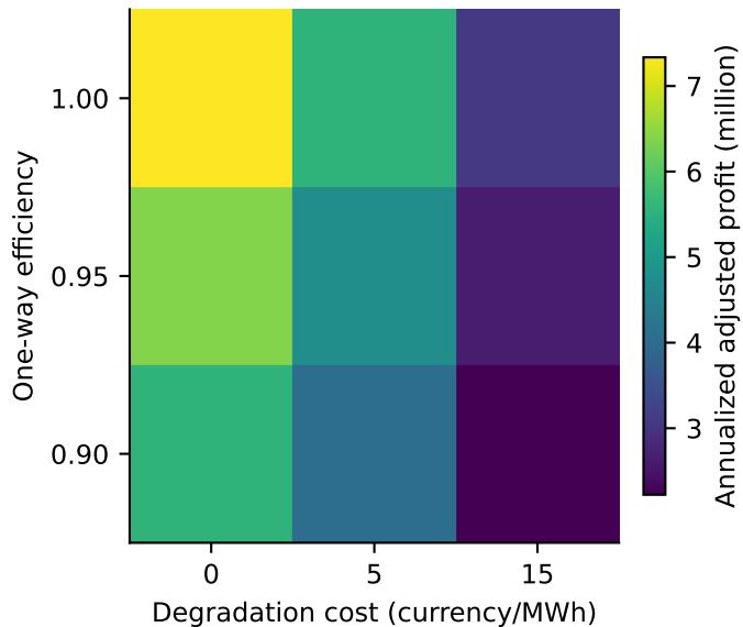
Synthetic seed 42
