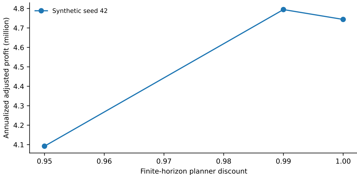
Planner-discount sensitivity; primary specification is \gamma = 1
