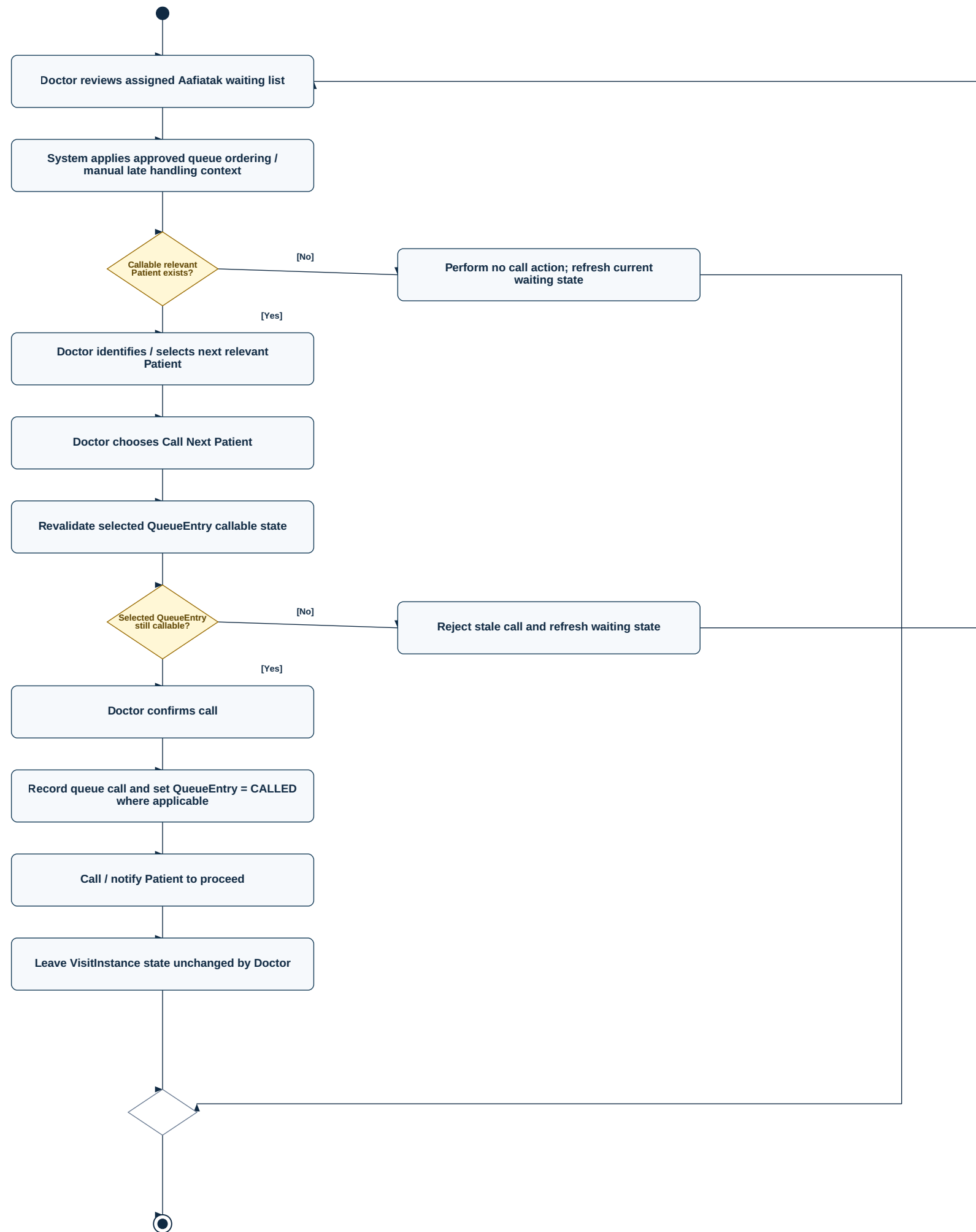
Activity Diagram — Call Next Patient
