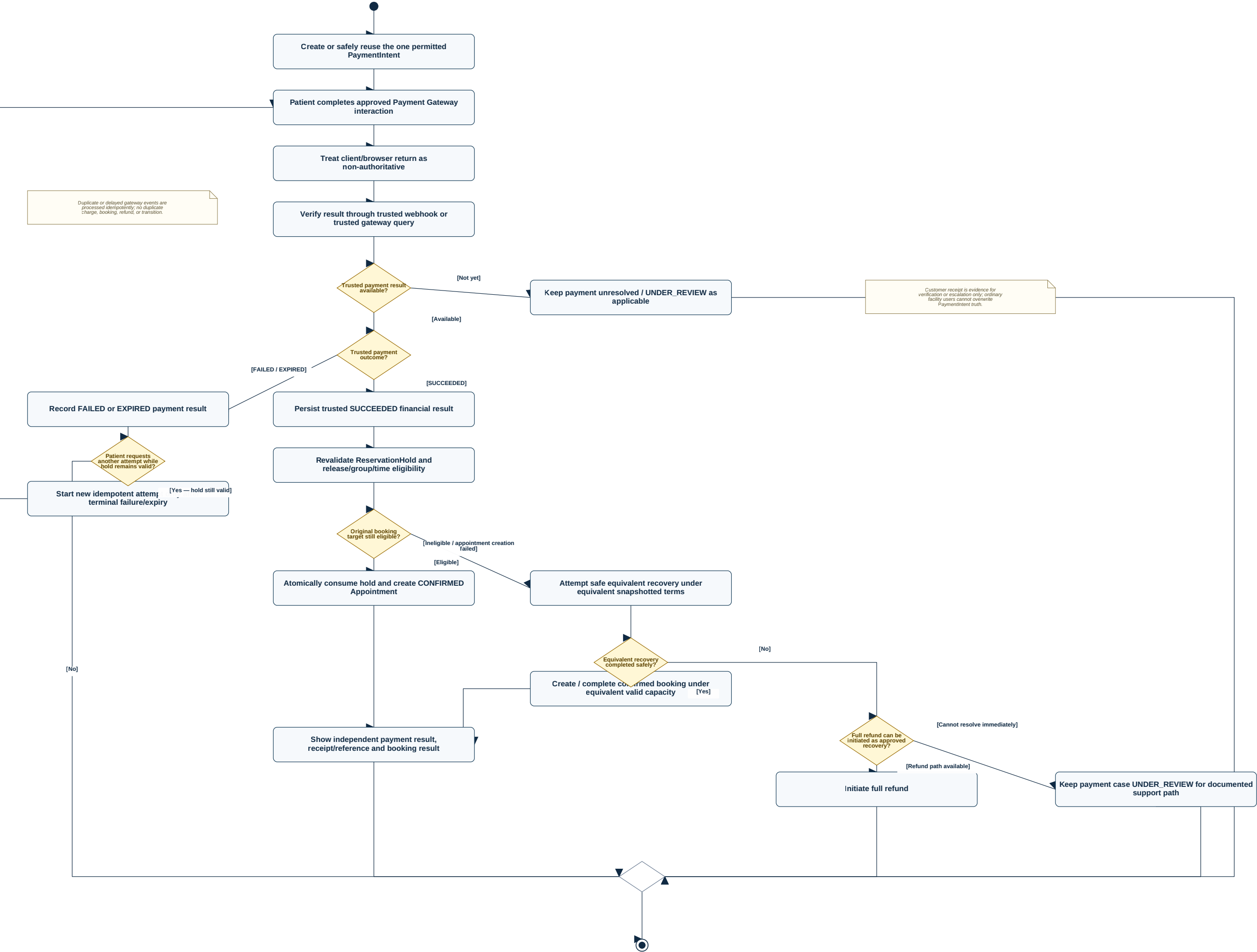
Activity Diagram — Process Full Payment
