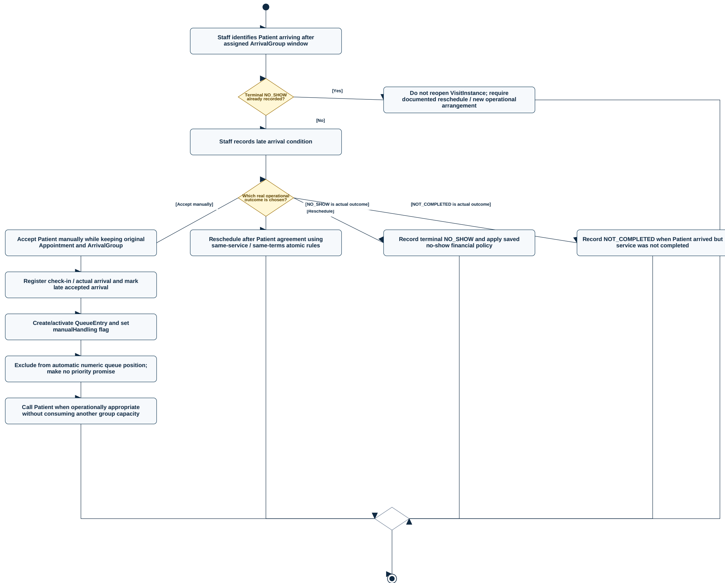
Activity Diagram — Handle Late Arrival
