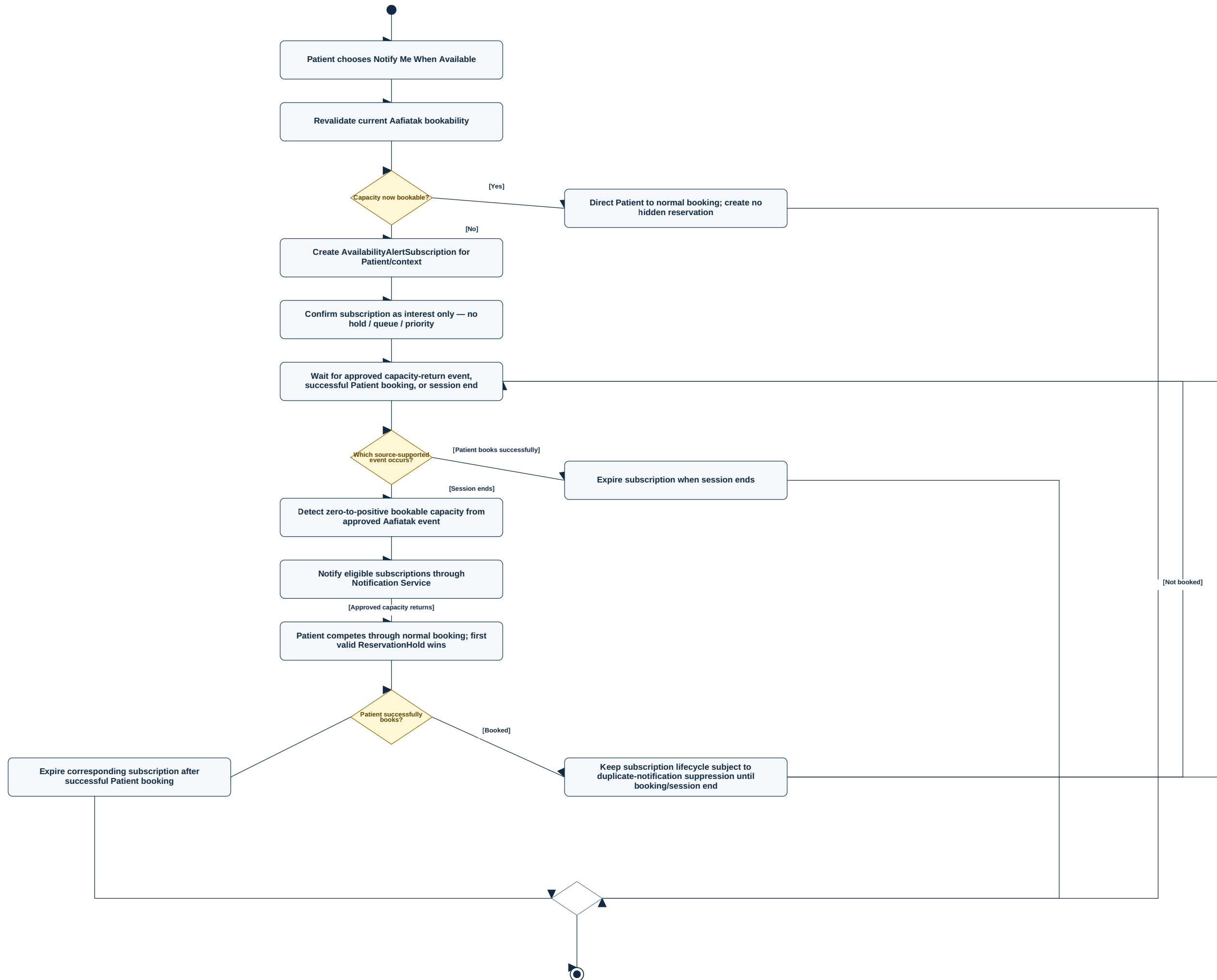
Activity Diagram — Subscribe to Availability Alert
