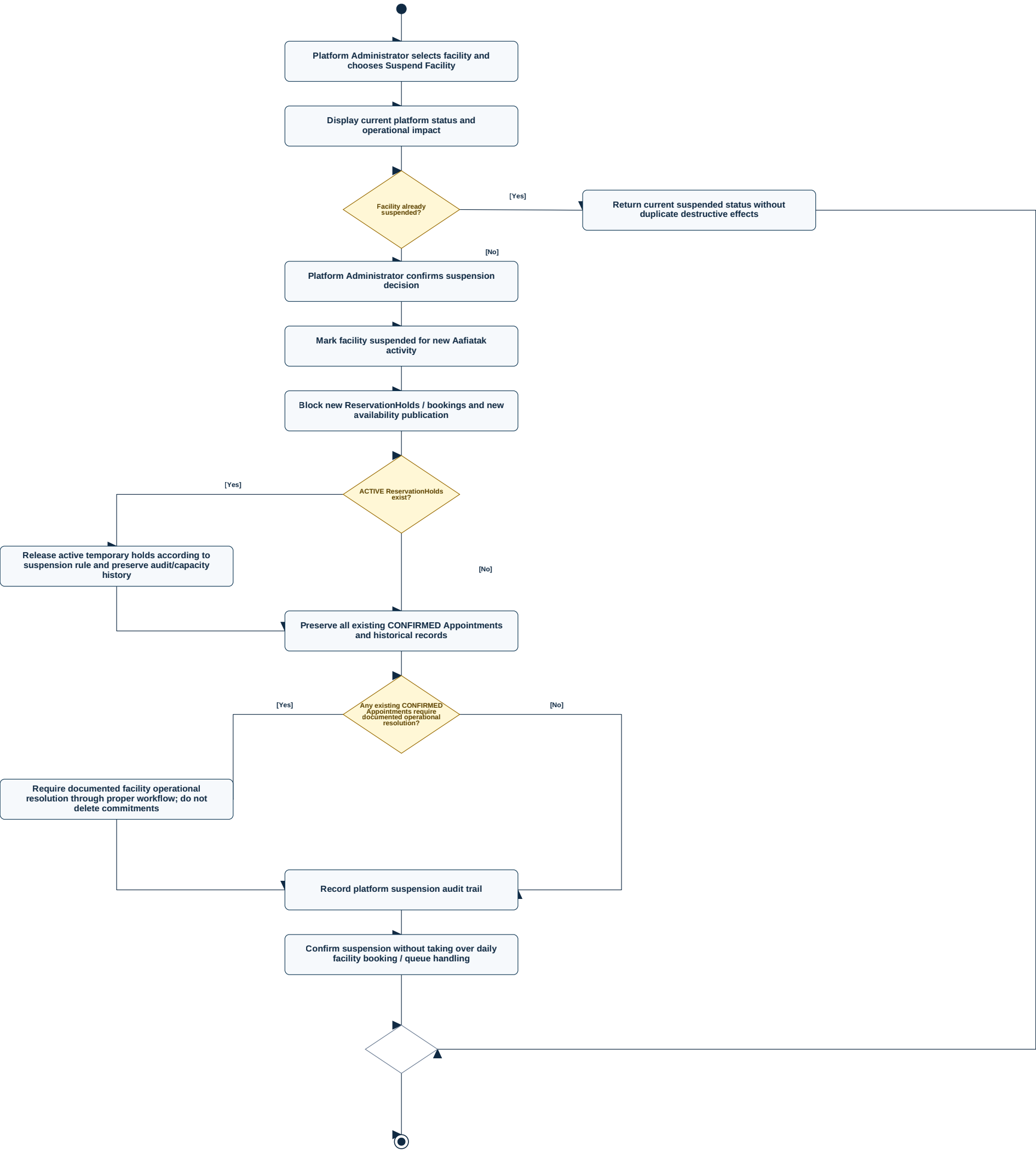
Activity Diagram — Suspend Facility
