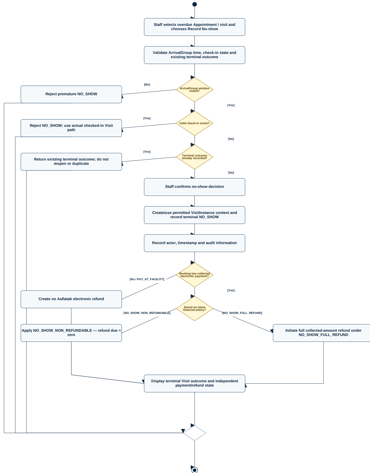
Activity Diagram — Record No-show
