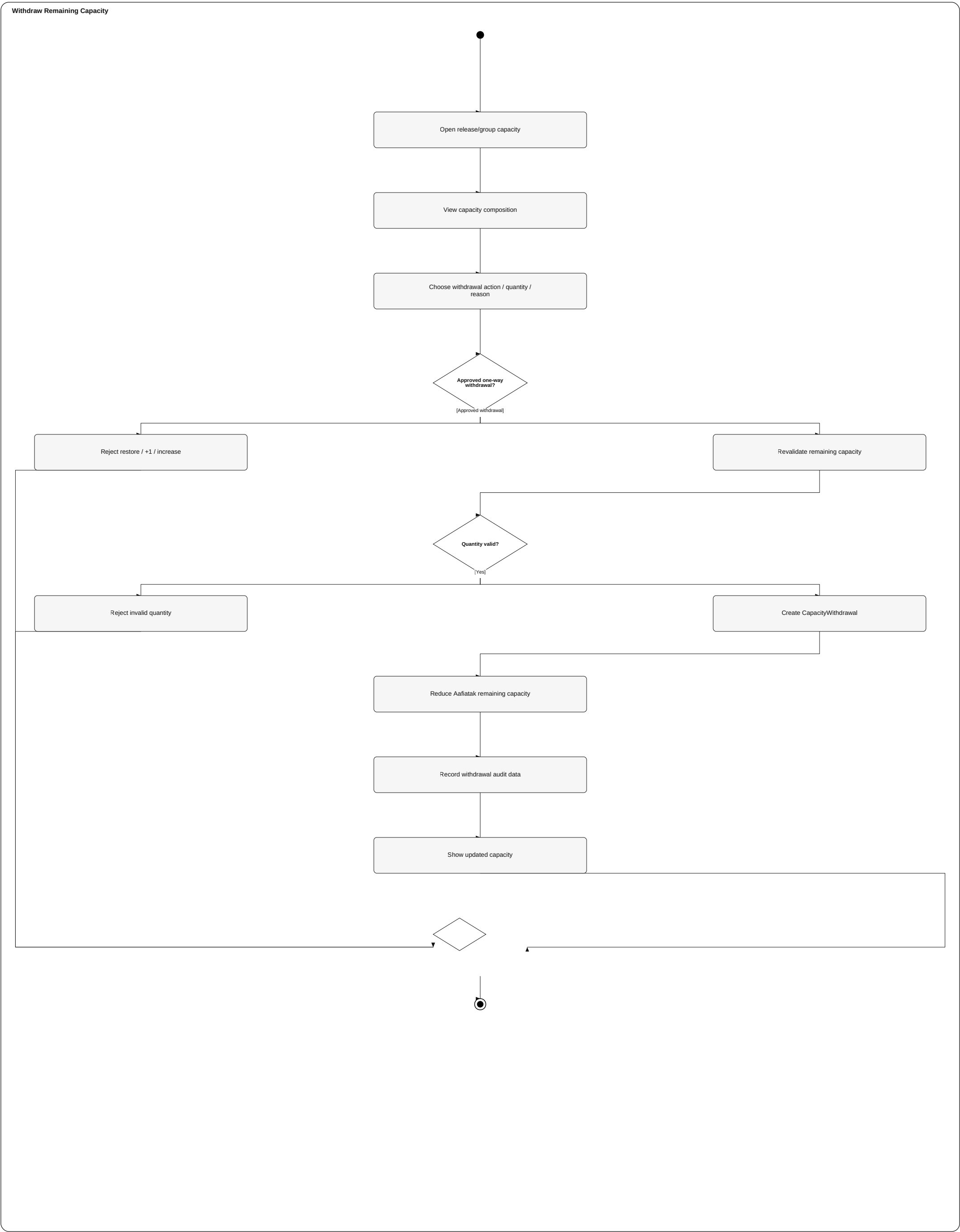
Activity Diagram — Withdraw Remaining Capacity
