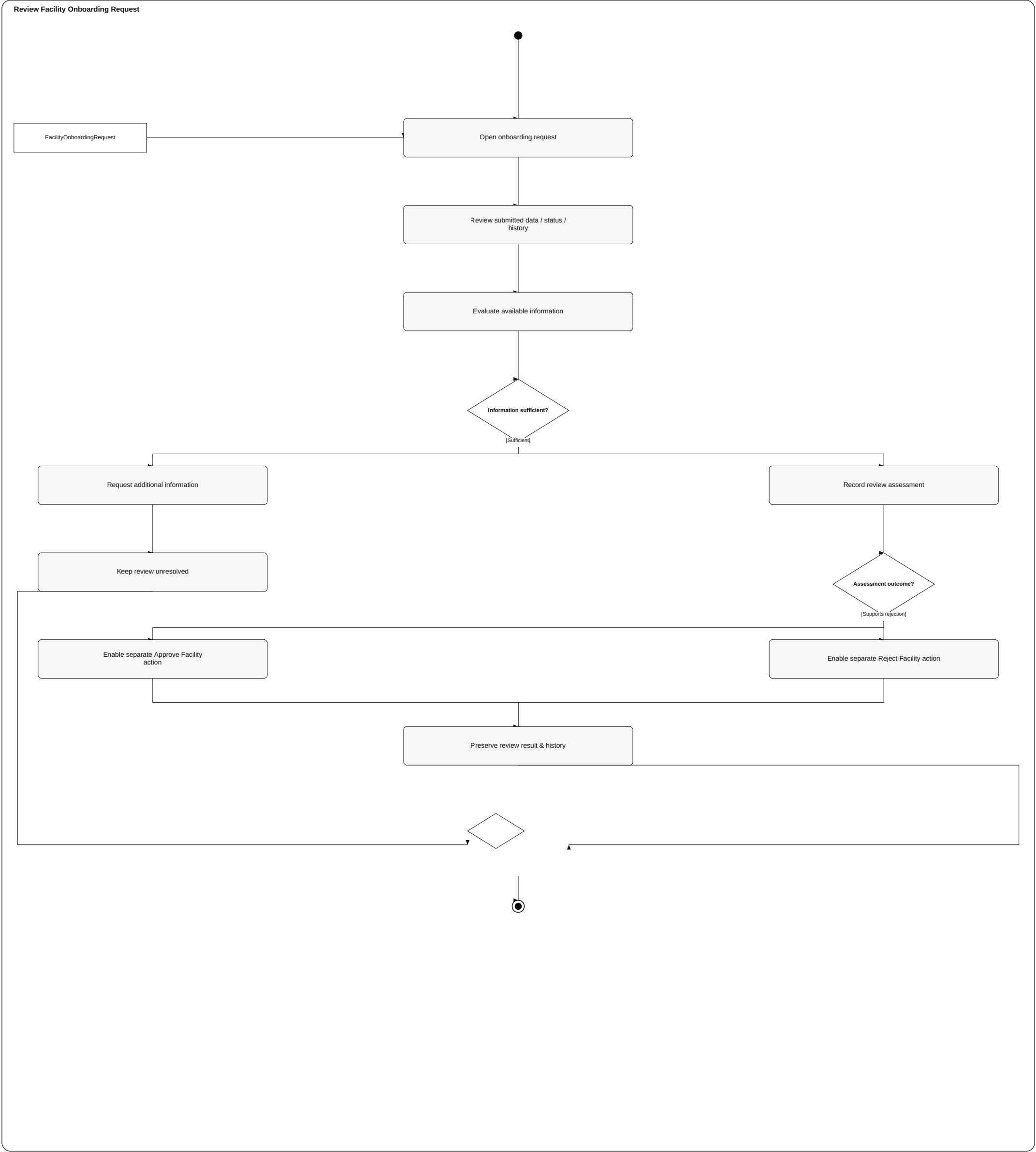
Activity Diagram — Review Facility Onboarding Request
