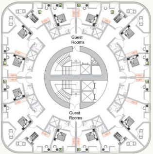
Guest-room floor plan - plan study
